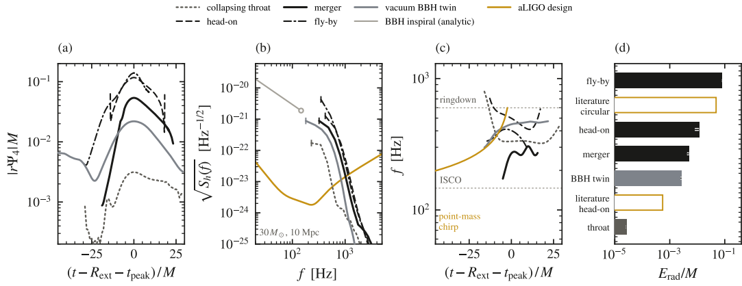
FIG. 8. Every source at one calibration: total mass 30 M_\odot at 10 Mpc, each record in units of its own total mass. (a) Upper envelopes of |r\Psi_4|/M at the innermost sphere, aligned at each peak: fly-by loudest ( 1.4 \times 10^{-1} ) to lone throat ( 3.1 \times 10^{-3} ). (b) Strain amplitude spectral densities over the aLIGO design floor (gold), each from its own low-frequency corner (one cycle per record, ticked). The curves are falling power laws (slopes -4.0 to -5.8 ) with no resolved maximum, so any “peak” read here is the corner 1/T . Faint line: the Newtonian inspiral of the same binary, |\dot{h}| \propto f^{-7/6} to its ISCO at 147 Hz. (c) Instantaneous frequency against the point-mass chirp (gold), the ISCO (147 Hz) and the equal-mass Kerr ringdown (599 Hz): the vacuum twin climbs the chirp and peaks at fM = 0.065 ; no wormhole channel does (Sec. IX A). (d) Energy radiated in the dominant multipole; ticks give the spread over spheres (head-on 30%, the widest). Open gold bars: published equal-mass vacuum values: head-on infall from rest at infinity, 5.5 \times 10^{-4} [87]; quasi-circular inspiral from infinite separation and merger, 4.84 \times 10^{-2} [81]; all multipoles. Energies are band integrals of |\int r\Psi_4 dt'|^2 over one retarded window per record, ending at its trust or noise gate (the lone throat’s at t = 58 , before its floor), at the spheres whose record covers it (the fly-by’s inner two), doubled for \pm m ; gravitational channel only. At 10^4 – 10^6 M_\odot and z_e \simeq 20 the same records are millihertz LISA sources (Sec. XB, Fig. 9). Movie of the vacuum twin: Video 7; youtu.be/NkcpGiJxXI .
