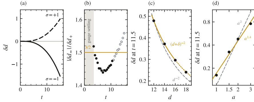
FIG. 4. Two throats at rest, on the far-side-matched pairs (Sec. IID): the sign rule (a,b), the force law (c) and its growth with throat width (d). (a) Separation change of two matched d = 12 pairs one sign apart: like-signed ( \sigma = +1 , dashed) opens, opposite-signed ( \sigma = -1 , solid) closes. Separations are inverse- \chi -weighted centroids of the midplane \chi pits. (b) Pull-to-push ratio against the prediction (Q+1)/(Q-1) = 3/2 (gold), where Q = |F_\phi/F_{\text{grav}}| = (a^2 + m^2)/m^2 = 5 is the scalar-to-gravity force ratio of Eq. (5): measured 1.462 \pm 0.022 (scatter over 15 slices); grey, the gauge-settling window t < 3.5 , excluded; open circles past t = 10.5 , where the closing pair has closed 4.6% of its gap, excluded too. (c) The force law on the ladder: how far like-signed pairs released from rest at d = 12/14/16/18 have pushed themselves apart by t = 11.5 (dots), against inverse-square in the coordinate separation scaled through d = 12 (grey, dashed) and A/(d + \delta)^2 fitted on d = 12 –16 alone (gold), dotted where it predicts the d = 18 rung (Sec. VB). If the push were inverse-square in d , every dot would lie on the grey curve; the dots rise above it, and the gold fit absorbs the excess with the offset \delta . (d) The push against throat width, on logarithmic axes: how far like-signed d = 12 pairs of width a = 1/1.5/2/3 have pushed themselves apart by t = 11.5 (dots; a = 2 is the d = 12 rung of (c)), against the point-charge a^2 of Eq. (5) scaled through a = 2 (grey, dashed) and a power law fitted to all four rungs (gold). If the push grew as a^2 , every dot would lie on the grey line; the dots climb more slowly, as a^{1.4} .
