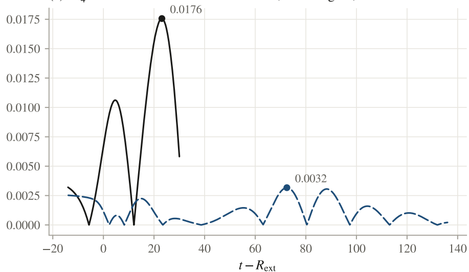
(c) |\Psi_4^{2,0}| — the wormholes' extra channel, 5.5 \times higher, 49 earlier
