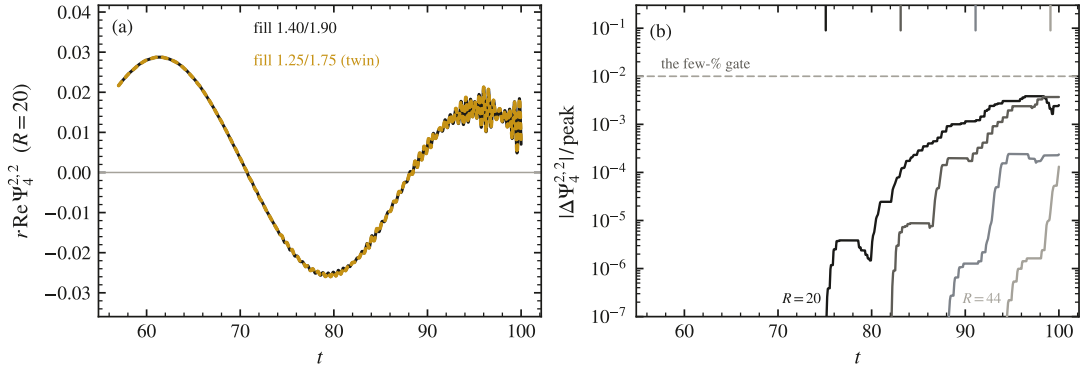
FIG. 13. Insensitivity of the spiral’s burst to the fill window. (a) r \text{Re} \Psi_4^{2,2} at R = 20 for the freeze arm (fill 1.40/1.90, ink) and its twin (1.25/1.75, gold dots) from the same t = 57 checkpoint. (b) Per-sphere envelope of the difference: at most 0.385% of peak at R = 20 and 0.013% at R = 44 , with ticks at the fill’s causal clock t = 57 + (R - 1.9) on each sphere. The difference reaches R = 20 on that clock and runs ahead of it farther out at 1.2–1.3 c (a gauge-speed front), below 1.5 \times 10^{-5} of peak. The outcome: moving the frozen region’s edge moves the waveform by under half a percent, and the burst, which peaks at R = 20 13 units before the core’s light cone arrives, cannot depend on the freeze at all.
