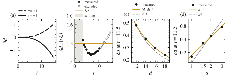
FIG. 5. Two throats at rest, on the far-side-matched pairs (Sec. IIID): the sign rule (a,b), the force law (c) and its growth with throat width (d). (a) Separation change of two matched d = 12 pairs one sign apart: like-signed ( \sigma = +1 , dashed) opens, opposite-signed ( \sigma = -1 , solid) closes. Separations are inverse- \chi -weighted centroids of the midplane \chi pits. (b) Pull-to-push ratio against the prediction (Q+1)/(Q-1) = 3/2 (gold), where Q = |F_\phi/F_{\text{grav}}| = (a^2 + m^2)/m^2 = 5 is the scalar-to-gravity force ratio of Eq. (5): measured 1.462 \pm 0.022 (scatter over 15 slices); grey, the gauge-settling window t < 3.5 , excluded; open circles past t = 10.5 , where the closing pair has closed 4.6% of its gap, excluded too. (c) The force law on the ladder: how far like-signed pairs released from rest at d = 12/14/16/18 have pushed themselves apart by t = 11.5 (dots), against inverse-square in the coordinate separation scaled through d = 12 (grey, dashed) and A/(d + \delta)^2 fitted on d = 12 –16 alone (gold), dotted where it predicts the d = 18 rung (Sec. VB). If the push were inverse-square in d , every dot would lie on the grey curve; the dots rise above it, and the gold fit absorbs the excess with the offset \delta . (d) The push against throat width, on logarithmic axes: how far like-signed d = 12 pairs of width a = 1/1.5/2/3 have pushed themselves apart by t = 11.5 (dots; a = 2 is the d = 12 rung of (c)), against the point-charge a^2 of Eq. (5) scaled through a = 2 (grey, dashed) and a power law fitted to all four rungs (gold). If the push grew as a^2 , every dot would lie on the grey line; the dots climb more slowly, as a^{1.4} .
