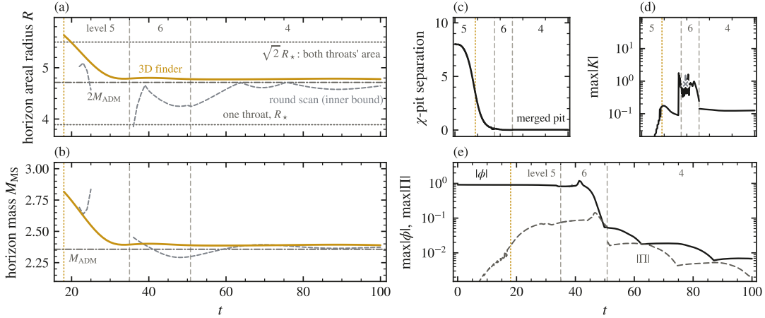
FIG. 6. The head-on merger ( d = 8 from rest, p = 0 , opposite signs) on matched, solved data ( M_{\text{ADM}} = 2.3573 ), and the black hole it makes. One evolution in three legs (faint dashed rules at the seams, t = 35 and 50.8 ; levels named in each panel; Sec. VIB): level 5 to a NaN in h_{11} at the merged core at t = 38.845 , inside the MOTS (its overrun grey to the death cross in (c)–(e)); level 6 from leg 1’s t = 35 checkpoint through the failure window; level 4 to t = 100 with no NaN. In-code \Psi_4 is identical on both overlaps. (a) Areal radius and (b) Misner–Sharp mass of the common MOTS. Gold: the spectral finder’s history (Sec. IIID, one row per plotfile, the three replay legs joined), born at t = 18 with R = 5.634 ( M_{\text{MS}} = 2.817 ) and shrinking—regrowing by at most 0.34%—toward the Schwarzschild sphere of the pair’s mass: R = 4.7787 and M_{\text{MS}} = 2.3894 at t = 100 , 1.4% above 2M_{\text{ADM}} and 1.4% above M_{\text{ADM}} . Grey dashes: the round star scan, the inner bound of Sec. IIID, late and small at birth and blind over t = 26 –35 (Sec. VIA). Rules: one isolated throat, R_* = 3.8895 ; \sqrt{2}R_* , a sphere with both throats’ area; 2M_{\text{ADM}} ( M_{\text{ADM}} in (b)). (c) Separation of the \chi pits. (d) \max|K| . (e) Grid maxima of |\phi| (solid) and |\text{II}| (dashed): the field is swallowed. Gold dotted rule: horizon birth. Movie: Video 3; youtu.be/3sx9GHRTYVs .
