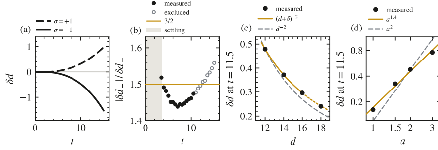
FIG. 5. Two throats at rest, on the far-side-matched pairs (Sec. IIID): the sign rule (a,b), the force law (c) and its growth with throat width (d). (a) Separation change of two matched d = 12 pairs one sign apart: like-signed ( \sigma = +1 , dashed) opens, opposite-signed ( \sigma = -1 , solid) closes. Separations are inverse- \chi -weighted centroids of the midplane \chi pits. (b) Pull-to-push ratio against the prediction (Q+1)/(Q-1) = 3/2 (gold), where Q = |F_\phi/F_{\text{grav}}| = (a^2 + m^2)/m^2 = 5 is the scalar-to-gravity force ratio of Eq. (5): measured 1.462 \pm 0.022 (scatter over 15 slices); grey, the gauge-settling window t < 3.5 , excluded; open circles past t = 10.5 , where the closing pair has closed 4.6% of its gap, excluded too. (c) The force law on the ladder: how far like-signed pairs released from rest at d = 12/14/16/18 have pushed themselves apart by t = 11.5 (dots), against inverse-square in the coordinate separation scaled through d = 12 (grey, dashed) and A/(d + \delta)^2 fitted on d = 12 –16 alone (gold), dotted where it predicts the d = 18 rung (Sec. VB). If the push were inverse-square in d , every dot would lie on the grey curve; the dots rise above it, and the gold fit absorbs the excess with the offset \delta . (d) The push against throat width, on logarithmic axes: how far like-signed d = 12 pairs of width a = 1/1.5/2/3 have pushed themselves apart by t = 11.5 (dots; a = 2 is the d = 12 rung of (c)), against the point-charge a^2 of Eq. (5) scaled through a = 2 (grey, dashed) and a power law fitted to all four rungs (gold). If the push grew as a^2 , every dot would lie on the grey line; the dots climb more slowly, as a^{1.4} .
