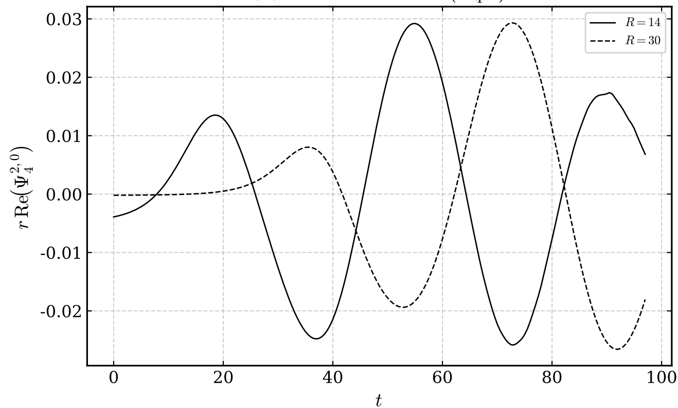
(a) Waveform r \text{Re}(\Psi_4^{2,0})
