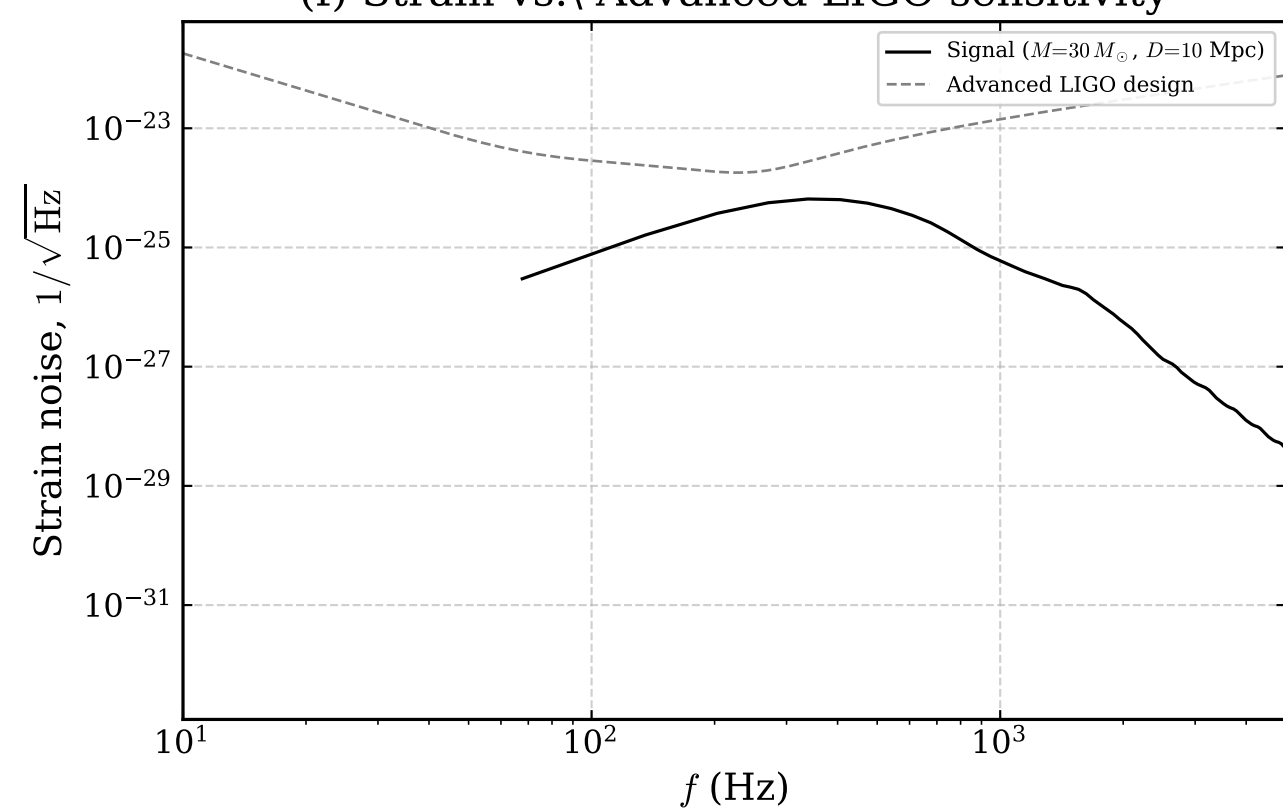
(f) Strain vs. Advanced LIGO sensitivity
