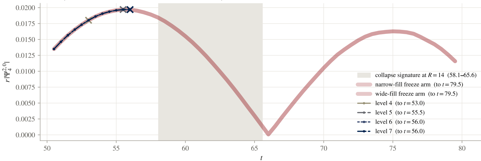
(b) axisymmetric channel (\ell, m) = (2, 0) — the head-on-style burst
