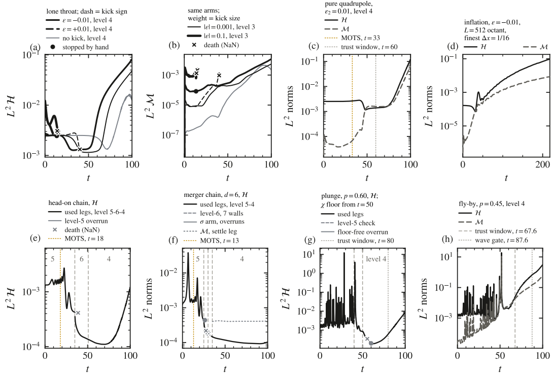
FIG. 12. Constraint evolution of every run the main-text figures draw, each at the highest refinement level it was run at (named in each panel's key): L^2 norms of the Hamiltonian ( \mathcal{H} , ink) and momentum ( \mathcal{M} , grey dashed) constraints, box averages on the base grid ( \Delta x = 0.5 ; 2 on the octant of (d)) that compare only within one box (Sec. III C). (a),(b) The lone throat of Fig. 3: level 4 for the unkicked throat and \varepsilon = \pm 10^{-2} ( +10^{-2} stopped by hand, dot), level 3 for \pm 10^{-3} and \pm 0.1 (dash = sign, weight = amplitude, grey = no kick, crosses = deaths). At t = 0 the norms carry the exact data's discretisation floor plus the kick's own defect, 0.090 |\varepsilon| (Sec. II F), which feeds \mathcal{M} within the first steps; the |\varepsilon| \leq 10^{-2} arms then follow the unkicked norms to 5.4% until the fates part, while \varepsilon = \pm 0.1 starts 3\text{--}6\times high and dies in a one-step overflow at the compactified origin. (c) The pure-quadrupole collapse of Fig. 4 (gold, its MOTS from t = 33 ; dotted, its trust window, t = 60 ): the late rise comes after it. (d) The inflating throat of Fig. 4 to t = 218 . (e) The head-on chain of Fig. 6 with its ladder (era rules at the restarts, levels per era): the level-5 segment's overrun dies of the censored interior NaN at t = 38.845 (cross) with its norm below its value at formation (gold rule, t = 18 ). (f) The d = 6 merger chain of Fig. 7: the used segments in ink, every failed arm in grey to its death cross (the level-6 and level-7 restarts dashed; times in Fig. 7(d)). At every end, hand stop and death alike, the Hamiltonian norm sits at or below its start: each failure is the interior NaN of Sec. VII D, not a constraint blow-up. (g) The p = 0.60 plunge, level 4 throughout: the floor-free extension (grey) dies of the merged core's cell NaN at t = 55.5 with its norm at its floor, the \chi -floor segment carries the record to t = 100 , and a level-5 restart (grey dashed) crosses the merger with clean norms; dotted, the trust window ( t = 80 ). (h) The p = 0.45 fly-by: the norms sit on their floor through the pass and grow as the mouths inflate; rules, the trust window ( t = 67.6 ) and the energy integral's end ( t = 87.6 ). The spikes on (g), (h) and the p = 0.25 arm, never on the head-on or d = 6 chains, are the base-grid norm reading the moving throats' \chi pits: on the p = 0.25 verification pair four cells next to the pits carry 99.99% of a spike while the level-3 solution is clean, and neither \max |K| nor the waves carry a counterpart.
