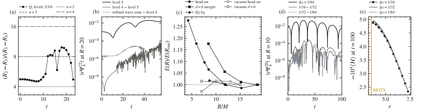
FIG. 11. Convergence. (a) The static throat from exact data at levels 2–4: the three-level factor Q = (R_2 - R_3)/(R_3 - R_4) of its minimal areal radius against the orders n = 2, 3, 4 (rules); the dip at t = 16 is one level-2 dump. (b) Bowen–York, not production, data: |r\Psi_4^{22}| at R = 20 of the d = 12 , p = 0.12 pair at throat level 5, its difference from level 4, and the difference made by refining the wave zone to half the base cell. (c) Radiated energy on each sphere over the outermost sphere’s, against R/M : the head-on, the d = 6 merger and the fly-by (ink) and two vacuum controls (grey). (d) The far-zone head-on of Fig. 8(b) at finest \Delta x = 1/16, 1/32 and 1/64 : |r\Psi_4^{20}| at R = 10 and each neighbouring pair’s difference, peaking at 0.55% and 0.54% of the peak. All three form the common MOTS at t = 18 , its R and M_{\text{MS}} equal between neighbouring levels to at most 0.08%, and the energy at R = 10 converges at order 1.7: differences 0.3%, then 0.09%. (e) The same three runs’ t = 100 checkpoints: shell averages of \mathcal{H}_{\text{ADM}} against r outside the common MOTS (gold rule, its largest coordinate extent), read on the shared level-4 grid; each halving of the interior cell moves them by 1.4%, then 0.4%. The outcome: orders 3.0–3.3 (static throat; 2.2–2.3 while its seed dominates), 1.7 (head-on energy) and 1.7 ( \mathcal{H}_{\text{ADM}} ); a binary’s waveform is resolved to 0.4% of its peak, the energy converges in extraction radius and in resolution, and the interior’s constraint violation does not leak past the horizon.
