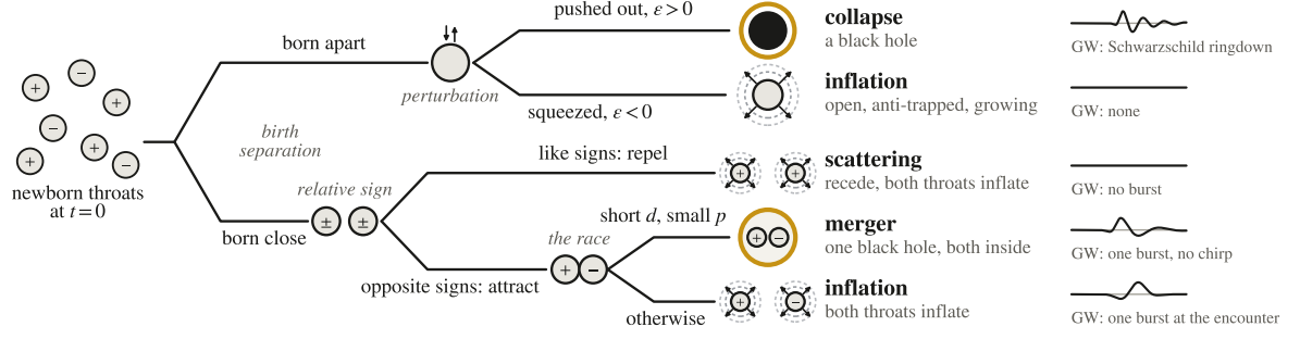
FIG. 1. Fates of newborn throats, whatever their origin, schematic: a lone throat’s perturbation sign selects collapse or inflation (Sec. IV C), a pair’s relative sign repulsion or attraction (Sec. V A), a repelling pair’s throats inflate as it recedes (Sec. V C), and an attracting pair merges where its horizon outruns inflation (Sec. VII B). Gold: horizons; right: sketched wave signals. The outcome: two fates end in a black hole, each after a single chirpless burst; in every other fate the throats inflate.
