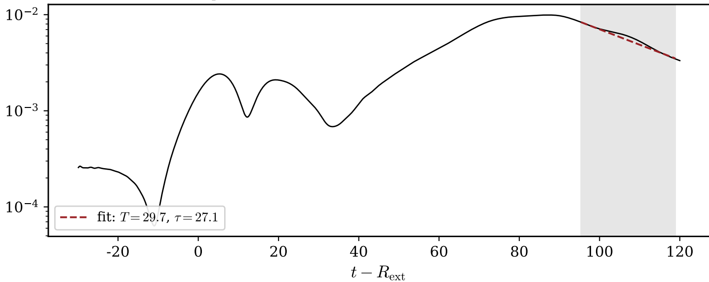
(b) |\Psi_4^{2,2}| envelope and exponential ringdown fit
