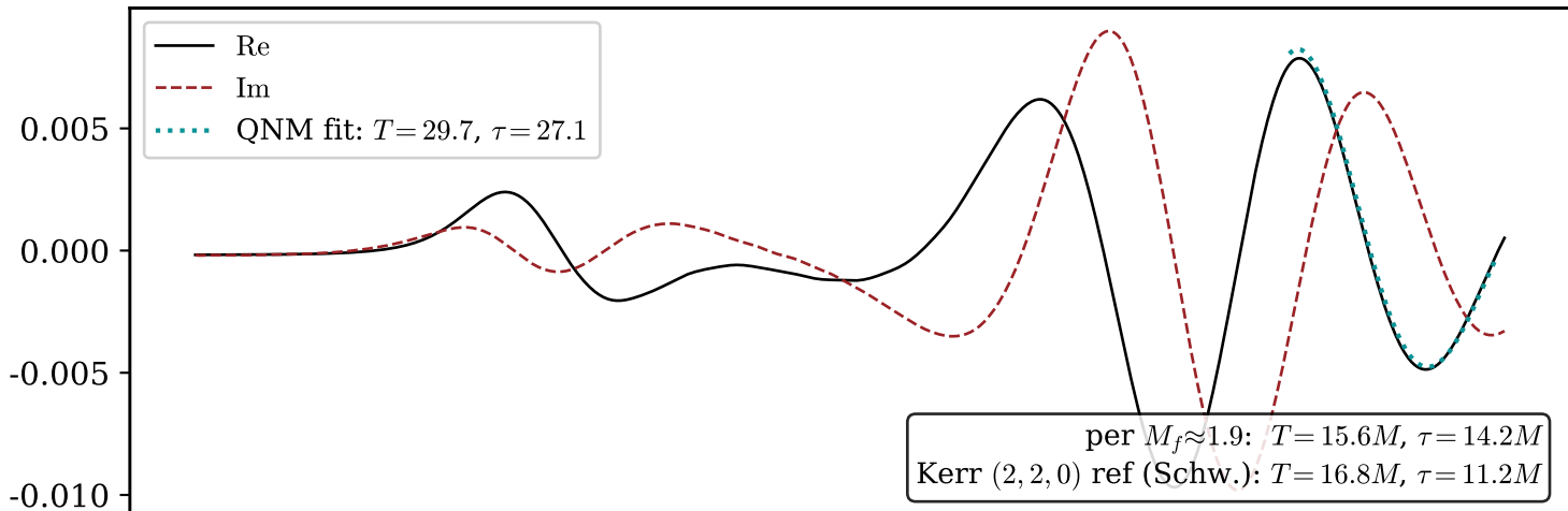
(a) \Psi_4^{2,2} mode at R=30 , BBH control to t=150
