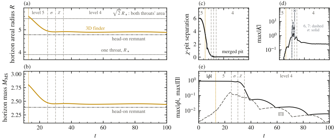
FIG. 7. The orbital merger ( d = 6 , tangential p = 0.10 , opposite signs, boosted mode-3 data) carried through its merger wall, and the black hole it settles to. One evolution composed across its legs (faint dashed rules at the restarts, t = 25, 30 and 35 ; levels named in the panels, \sigma and \chi for the two wall legs): level 5 from t = 0 , stopped at t = 26.26 as the merged core's K ran away; the \sigma_{\text{KO}} = 1.0 leg; the \chi -floor crossing leg; the level-4 settle leg to t = 100 , no NaN. (a) Areal radius and (b) Misner–Sharp mass of the common MOTs: gold, the spectral finder's history (Sec. III D), born at t = 13 and falling from above toward the head-on remnant's values (dash-dotted rules, R = 4.7787 ; M_{\text{MS}} = 2.3894 in (b)). Dotted rules in (a): one isolated throat, R_* ; \sqrt{2}R_* , both throats' area. (c) Separation of the \chi pits (grey: leg 1's overrun past its restart checkpoint). (d) The wall: \max |K| of every arm—the used legs in ink; the level-6 and level-7 diagnostic restarts (grey dashed) die at t = 29.4 and, earlier, 27.5 , each an h_{11} NaN at the core's centre with the global norms clean to the last step; the \sigma arm (grey solid) clears the K wall and dies at the same cell at t = 30.5 (death crosses); the \chi -floor and settle legs carry the history through. (e) Grid maxima of |\phi| (solid) and |\text{II}| (dashed): the field is swallowed. Gold dotted rule: horizon birth. Movie: Video 7; youtu.be/jNnMAXPjyRA .
