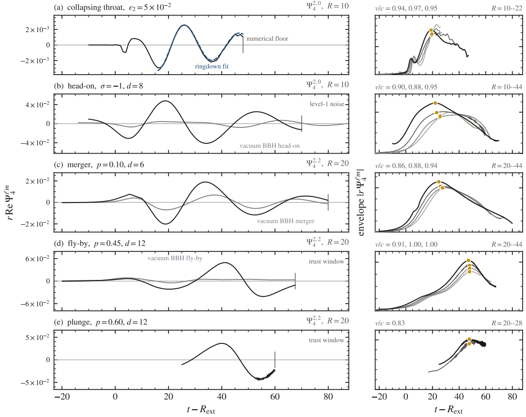
FIG. 7. The waveform gallery: one row per scenario on one retarded clock. Left: r \operatorname{Re} \Psi_4 of the dominant mode at the innermost sphere, each row on its own scale; row (a) is the \varepsilon_2 = 0.05 arm, with the ringdown fit of Sec. VIII A dashed (period 20.6 M ). Caps mark where the drawn record ends: the collapsing throat before its numerical floor exceeds 14% of the burst peak; the head-on where the noise of its level-1 refinement cube reaches the sphere (from t = 80 at R \leq 20 ); the fly-by at its trust window ( t - R = 67.6 ), the plunge at its own. The merger runs through remnant ringdown, with one linear bridge across a leg seam. Grey under (b)–(d): the vacuum controls, black holes at the same d and p on bare punctures, on the same scale: the vacuum head-on rings 5.4\times lower and crests later (Sec. VIII B); the vacuum merger peaks at the drainhole merger’s retarded time, 3.0\times lower; the vacuum fly-by radiates one cycle as the holes swing away from periapsis, 6.7\times below the fly-by’s arch. Right: the amplitude envelope at every sphere on its own retarded time (ink to faint, inner to outer)—the upper envelope of |r \Psi_4| for the complex (2, 2) modes, the analytic-signal envelope for the real (2, 0) modes—which folds onto one curve for a signal moving at c and falling as 1/r . Gold dots: the correlated wavefront. The quoted v/c is the whole-waveform lag between neighbouring spheres (Sec. VIII E), the plunge’s the burst-peak lag: throat 0.94/0.97/0.95, head-on 0.90/0.88/0.95, merger 0.86/0.88/0.94, fly-by 0.91/1.00/1.00, plunge 0.83. Movies of the vacuum head-on and fly-by: Videos 8 youtu.be/aRWvD4W8Oog and 9 youtu.be/65_3kw4obvE .
