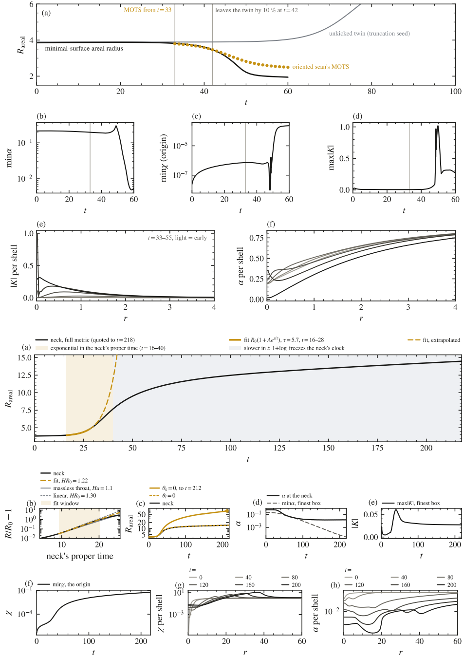
FIG. 3. Top (collapse branch): Collapse of the pure-quadrupole arm ( \varepsilon_2 = 0.01 , no radial kick). (a) Minimal-surface areal radius (ink) and the scan's MOTS (gold) from t = 33 to 60 : R 3.80 \rightarrow 2.50 , M_{\text{MS}} 1.90 \rightarrow 1.25 . Grey: the unkicked level-4 twin, which inflates on its own seed; this arm leaves it by 10% only at t = 42 —the second-order drive of the pure quadrupole. (b)–(d) Global \min \alpha , \min \chi (the origin, the far side's compactified infinity) and \max |K| ; the violent phase spans t = 45 – 55 . (e), (f) Radial profiles over 128 shells, t = 33 – 55 (light = early): |K| grows inward while \alpha pinches to zero at the centre. Constraint norms: Fig. 11(c). The collapse ends in a black hole that consumes its supporting field. Movie: Video 1; youtu.be/Cc87mHcBPOA . Bottom (inflation branch): The inflating throat ( \varepsilon = -10^{-2} ; L = 512 octant, finest \Delta x = 1/16 ) to t = 218 . (a) Neck areal radius in the full metric, 3.81 \rightarrow 14.5 ; gold, the exponential onset, \tau = 5.7 over t = 16 – 28 ; shaded, exponential growth in the neck's proper time ( t = 16 – 40 , gold) and the slower growth in t once 1 + \log freezes the neck's clock (grey). (b) Over that window the neck's proper-time rate is HR_0 = 1.22 (local 1.0 – 1.3 ), against the massless throat's Ha = 1.1 [13] and the linear mode's 1.30 . (c) The \theta_l = 0 horizon stays on the neck; \theta_k = 0 runs out to R \approx 73 by t = 212 . (d) The lapse at the neck falls 0.57 \rightarrow 0.015 ; dashed, its minimum on the finest box. (e), (f) \max |K| and \min \chi on the finest box, around the origin. (g), (h) \chi and \alpha per shell (light = early): the \chi peak moves out with the neck. Constraint norms: Fig. 11(d). The throat keeps growing, anti-trapped. Movie: Video 2; youtu.be/RIQCitu4tSc .
