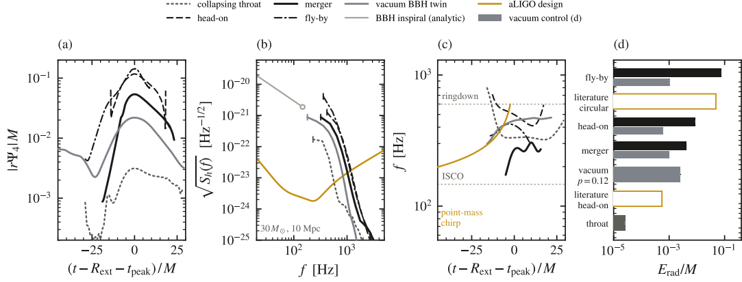
FIG. 8. Every source at one calibration: total mass 30 M_\odot at 10 Mpc, each record in units of its own total mass; the vacuum twin is two black holes with the separation and momentum of the d = 12 , p = 0.12 arm (Sec. VII A). (a) Upper envelopes of |r\Psi_4|/M at the innermost sphere, aligned at each peak: fly-by loudest ( 1.4 \times 10^{-1} ) to lone throat ( 3.1 \times 10^{-3} ). (b) Strain amplitude spectral densities over the aLIGO design floor (gold), each from its own low-frequency corner (one cycle per record, ticked). The curves are falling power laws (slopes -4.0 to -5.8 ) with no resolved maximum, so any “peak” read here is the corner 1/T . Faint line: the Newtonian inspiral of the same binary, |\dot{h}| \propto f^{-7/6} to its ISCO at 147 Hz. (c) Instantaneous frequency against the point-mass chirp (gold), the ISCO (147 Hz) and the equal-mass Kerr ringdown (599 Hz): the vacuum twin climbs the chirp and peaks at fM = 0.065 ; no wormhole channel does (Sec. IX A). (d) Energy radiated in the dominant multipole at the outermost sphere covering each record’s window, the tick its change from the next sphere in; grey under each source, its vacuum control at the same d and p . Open gold bars: published equal-mass vacuum values: head-on infall from rest at infinity, 5.5 \times 10^{-4} [87]; quasi-circular inspiral from infinite separation and merger, 4.84 \times 10^{-2} [81]; all multipoles. Energies are band integrals of |\int r\Psi_4 dt|^2 over one retarded window per record, ending at its trust or noise gate (the lone throat’s at t = 58 , before its floor), at the spheres whose record covers it (the fly-by’s inner two), doubled for \pm m ; gravitational channel only. At 10^4 – 10^6 M_\odot and z_e \simeq 20 the same records are millihertz LISA sources (Sec. XB, Fig. 9). Movie of the vacuum twin: Video 10; youtu.be/NkcpGjIIXI .
