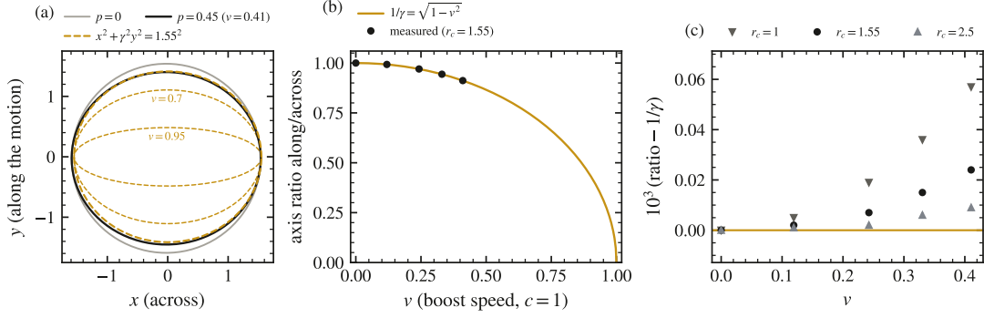
FIG. 1. The moving throat at t = 0 is the Lorentz-contracted drainhole. (a) The \chi contour just inside the throat, at rest and at p = 0.45 , the latter on its analytic ellipse; the fainter ellipses continue the law to v = 0.7 and 0.95 . (b) Axis ratio (along/across the motion) against the boost speed v = p/\sqrt{m^2 + p^2} , on 1/\gamma = \sqrt{1 - v^2} drawn to the disc limit v = 1 . (c) The residual: below 6 \times 10^{-5} at every v and at three contour levels. The outcome: the boosted data carry exactly the special-relativistic shape, with the scalar in motion, and both constraints hold at the exact solution’s discretisation floor.
