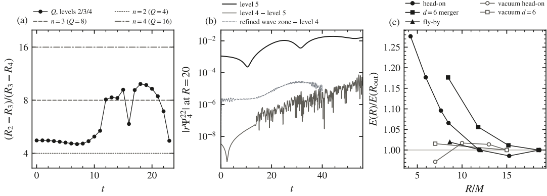
FIG. 10. Convergence. (a) The static throat from exact data at levels 2–4: the three-level factor Q = (R_2 - R_3)/(R_3 - R_4) of its minimal areal radius against the orders n = 2, 3, 4 (rules); the dip at t = 16 is one level-2 dump. (b) |r\Psi_4^{22}| at R = 20 of the d = 12 , p = 0.12 pair with Bowen–York momentum (otherwise our data) at throat level 5, its difference from level 4, and the difference made by refining the wave zone to half the base cell. (c) Radiated energy on each sphere over the outermost sphere’s, against R/M : the head-on, the d = 6 merger and the fly-by (ink) and two vacuum controls (grey). The outcome: the scheme converges at order 3.0–3.3, a binary’s waveform is resolved to 0.4% of its peak, and the energy converges in extraction radius.
