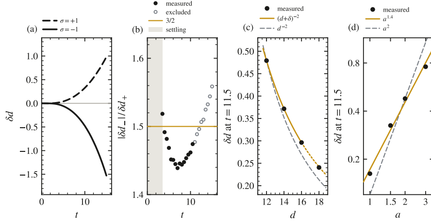
FIG. 4. Two throats at rest, on the far-side-matched pairs (Sec. IID): the sign rule (a,b), the force law (c) and its growth with throat width (d). (a) Separation change of two matched d = 12 pairs one sign apart: like-signed ( \sigma = +1 , dashed) opens, opposite-signed ( \sigma = -1 , solid) closes. Separations are inverse- \chi -weighted centroids of the midplane \chi pits. (b) Pull-to-push ratio against the prediction (Q+1)/(Q-1) = 3/2 (gold), where Q = |F_\phi/F_{\text{grav}}| = (a^2 + m^2)/m^2 = 5 is the scalar-to-gravity force ratio of Eq. (5): measured 1.462 \pm 0.022 (scatter over 15 slices); grey, the gauge-settling window t < 3.5 , excluded; open circles past t = 10.5 , where the closing pair has closed 4.6% of its gap, excluded too. (c) The force law on the ladder: how far like-signed pairs released from rest at d = 12/14/16/18 have pushed themselves apart by t = 11.5 (dots), against inverse-square in the coordinate separation scaled through d = 12 (grey, dashed) and A/(d + \delta)^2 fitted on d = 12\text{--}16 alone (gold), dotted where it predicts the d = 18 rung (Sec. VB). If the push were inverse-square in d , every dot would lie on the grey curve; the dots rise above it, and the gold fit absorbs the excess with the offset \delta . (d) The push against throat width, on logarithmic axes: how far like-signed d = 12 pairs of width a = 1/1.5/2/3 have pushed themselves apart by t = 11.5 (dots; a = 2 is the d = 12 rung of (c)), against the point-charge a^2 of Eq. (5) scaled through a = 2 (grey, dashed) and a power law fitted to all four rungs (gold). If the push grew as a^2 , every dot would lie on the grey line; the dots climb more slowly, as a^{1.4} .
