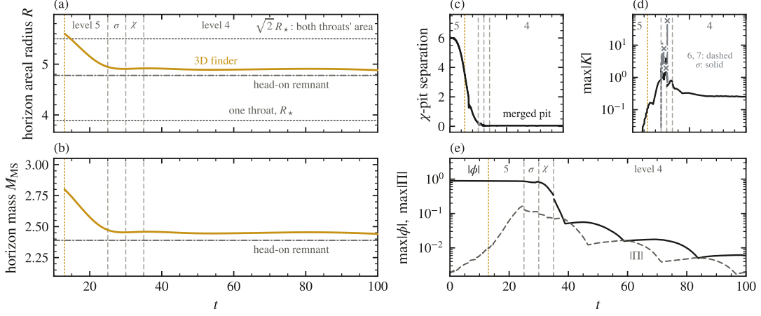
FIG. 7. The orbital merger ( d = 6 , tangential p = 0.10 , opposite signs, boosted mode-3 data) carried through its merger wall, and the black hole it settles to. One evolution composed across its legs (faint dashed rules at the restarts, t = 25, 30 and 35 ; levels named in the panels, \sigma and \chi for the two wall legs): level 5 from t = 0 , stopped at t = 26.26 as the merged core's K ran away; the \sigma_{\text{KO}} = 1.0 leg; the \chi -floor crossing leg; the level-4 settle leg to t = 100 , no NaN. (a) Areal radius and (b) Misner–Sharp mass of the common MOTs: gold, the spectral finder's history (Sec. III D), born at t = 13 and falling from above toward the head-on remnant's values (dash-dotted rules, R = 4.7787 ; M_{\text{MS}} = 2.3894 in (b)). Dotted rules in (a): one isolated throat, R_* ; \sqrt{2}R_* , both throats' area. (c) Separation of the \chi pits (grey: leg 1's overrun past its restart checkpoint). (d) The wall: \max |K| of every arm—the used legs in ink; the level-6 and level-7 diagnostic restarts (grey dashed) die at t = 29.4 and, earlier, 27.5 , each an h_{11} NaN at the core's centre with the global norms clean to the last step; the \sigma arm (grey solid) clears the K wall and dies at the same cell at t = 30.5 (death crosses); the \chi -floor and settle legs carry the history through. (e) Grid maxima of |\phi| (solid) and |\text{II}| (dashed): the field is swallowed. Gold dotted rule: horizon birth. Movie: Video 7; youtu.be/jNnMAXPjyRA .
