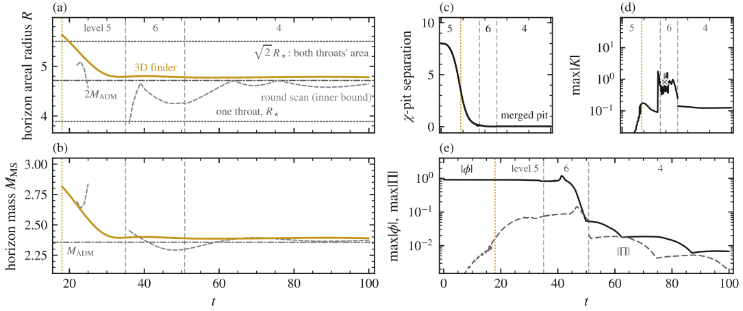
FIG. 6. The head-on merger ( d = 8 from rest, p = 0 , opposite signs) on matched, solved data ( M_{\text{ADM}} = 2.3573 ), and the black hole it makes. One evolution in three legs (faint dashed rules at the seams, t = 35 and 50.8 ; levels named in each panel; Sec. VIB): level 5 to a NaN in h_{11} at the merged core at t = 38.845 , inside the MOTS (its overrun grey to the death cross in (c)–(e)); level 6 from leg 1’s t = 35 checkpoint through the failure window; level 4 to t = 100 with no NaN. In-code \Psi_4 is identical on both overlaps. (a) Areal radius and (b) Misner–Sharp mass of the common MOTS. Gold: the spectral finder’s history (Sec. IIID, one row per plotfile, the three replay legs joined), born at t = 18 with R = 5.634 ( M_{\text{MS}} = 2.817 ) and shrinking—regrowing by at most 0.34\% —toward the Schwarzschild sphere of the pair’s mass: R = 4.7787 and M_{\text{MS}} = 2.3894 at t = 100 , 1.4\% above 2M_{\text{ADM}} and 1.4\% above M_{\text{ADM}} . Grey dashes: the round star scan, the inner bound of Sec. IIID, late and small at birth and blind over t = 26 – 35 (Sec. VIA). Rules: one isolated throat, R_* = 3.8895 ; \sqrt{2}R_* , a sphere with both throats’ area; 2M_{\text{ADM}} ( M_{\text{ADM}} in (b)). (c) Separation of the \chi pits. (d) \max|K| . (e) Grid maxima of |\phi| (solid) and |\text{II}| (dashed): the field is swallowed. Gold dotted rule: horizon birth. Movie: Video 3; youtu.be/3sx9GHRTYVs .
