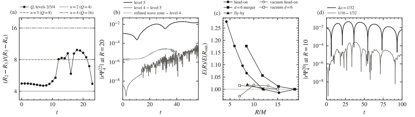
FIG. 11. Convergence. (a) The static throat from exact data at levels 2–4: the three-level factor Q = (R_2 - R_3)/(R_3 - R_4) of its minimal areal radius against the orders n = 2, 3, 4 (rules); the dip at t = 16 is one level-2 dump. (b) |r\Psi_4^{22}| at R = 20 of the d = 12, p = 0.12 pair with Bowen–York momentum (otherwise our data) at throat level 5, its difference from level 4, and the difference made by refining the wave zone to half the base cell. (c) Radiated energy on each sphere over the outermost sphere’s, against R/M : the head-on, the d = 6 merger and the fly-by (ink) and two vacuum controls (grey). (d) The far-zone head-on of Fig. 8(b) at finest \Delta x = 1/16 and 1/32 : |r\Psi_4^{20}| at R = 10 and the two levels’ difference, at most 0.5% of its peak. Both form the common MOTS at t = 18 , its R and M_{\text{MS}} equal to 0.08%, and their energies at R = 10 differ by 0.3%; a third level, \Delta x = 1/64 , so far run to t = 67 , shrinks that difference at order 1.7. The outcome: the scheme converges at order 3.0–3.3, a binary’s waveform is resolved to 0.4% of its peak, and the energy converges in extraction radius and in resolution.
