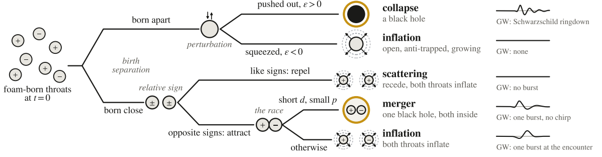
FIG. 1. Fates of foam-born throats, schematic: a lone throat’s perturbation sign selects collapse or inflation (Sec. IV C), a pair’s relative sign repulsion or attraction (Sec. V A), a repelling pair’s throats inflate as it recedes (Sec. V C), and an attracting pair merges where its horizon outruns inflation (Sec. VII B). Gold: horizons; right: sketched wave signals. The outcome: two fates end in a black hole, each after a single chirpless burst; in every other fate the throats inflate.
