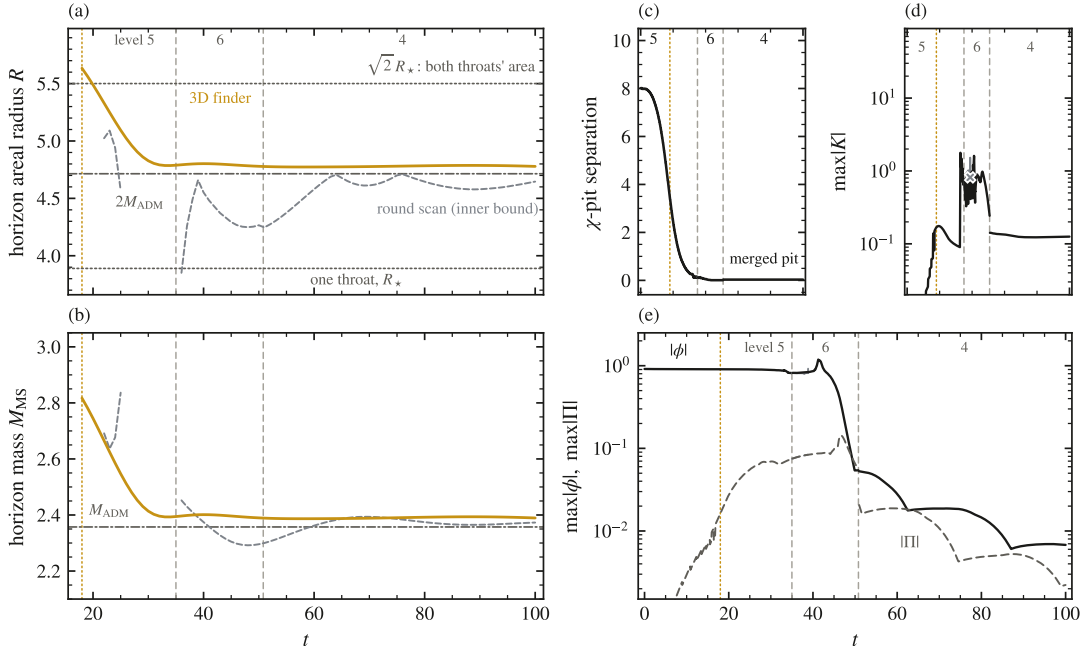
FIG. 6. The head-on merger ( d = 8 from rest, p = 0 , opposite signs) on matched, solved data ( M_{\text{ADM}} = 2.3573 ), and the black hole it makes. One evolution in three legs (faint dashed rules at the seams, t = 35 and 50.8 ; levels named in each panel; Sec. VIB): level 5 to a NaN in h_{11} at the merged core at t = 38.845 , inside the MOTS (its overrun grey to the death cross in (c)–(e)); level 6 from leg 1’s t = 35 checkpoint through the failure window; level 4 to t = 100 with no NaN. In-code \Psi_4 is identical on both overlaps. (a) Areal radius and (b) Misner–Sharp mass of the common MOTS. Gold: the spectral finder’s history (Sec. IIID, one row per plotfile, the three replay legs joined), born at t = 18 with R = 5.634 ( M_{\text{MS}} = 2.817 ) and shrinking—regrowing by at most 0.34\% —toward the Schwarzschild sphere of the pair’s mass: R = 4.7787 and M_{\text{MS}} = 2.3894 at t = 100 , 1.4\% above 2M_{\text{ADM}} and 1.4\% above M_{\text{ADM}} . Grey dashes: the round star scan, the inner bound of Sec. IIID, late and small at birth and blind over t = 26 – 35 (Sec. VIA). Rules: one isolated throat, R_* = 3.8895 ; \sqrt{2}R_* , a sphere with both throats’ area; 2M_{\text{ADM}} ( M_{\text{ADM}} in (b)). (c) Separation of the \chi pits. (d) \max|K| . (e) Grid maxima of |\phi| (solid) and |\text{II}| (dashed): the field is swallowed. Gold dotted rule: horizon birth. Movie: Video 3; youtu.be/3sx9GHRTYVs .
