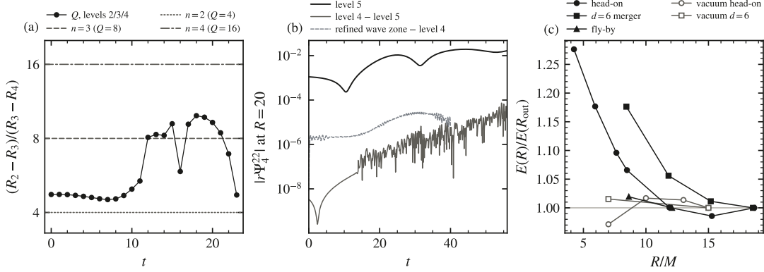
FIG. 11. Convergence. (a) The static throat from exact data at levels 2–4: the three-level factor Q = (R_2 - R_3)/(R_3 - R_4) of its minimal areal radius against the orders n = 2, 3, 4 (rules); the dip at t = 16 is one level-2 dump. (b) |r\Psi_4^{22}| at R = 20 of the d = 12, p = 0.12 pair with Bowen–York momentum (otherwise our data) at throat level 5, its difference from level 4, and the difference made by refining the wave zone to half the base cell. (c) Radiated energy on each sphere over the outermost sphere’s, against R/M : the head-on, the d = 6 merger and the fly-by (ink) and two vacuum controls (grey). The outcome: the scheme converges at order 3.0–3.3, a binary’s waveform is resolved to 0.4% of its peak, and the energy converges in extraction radius.
