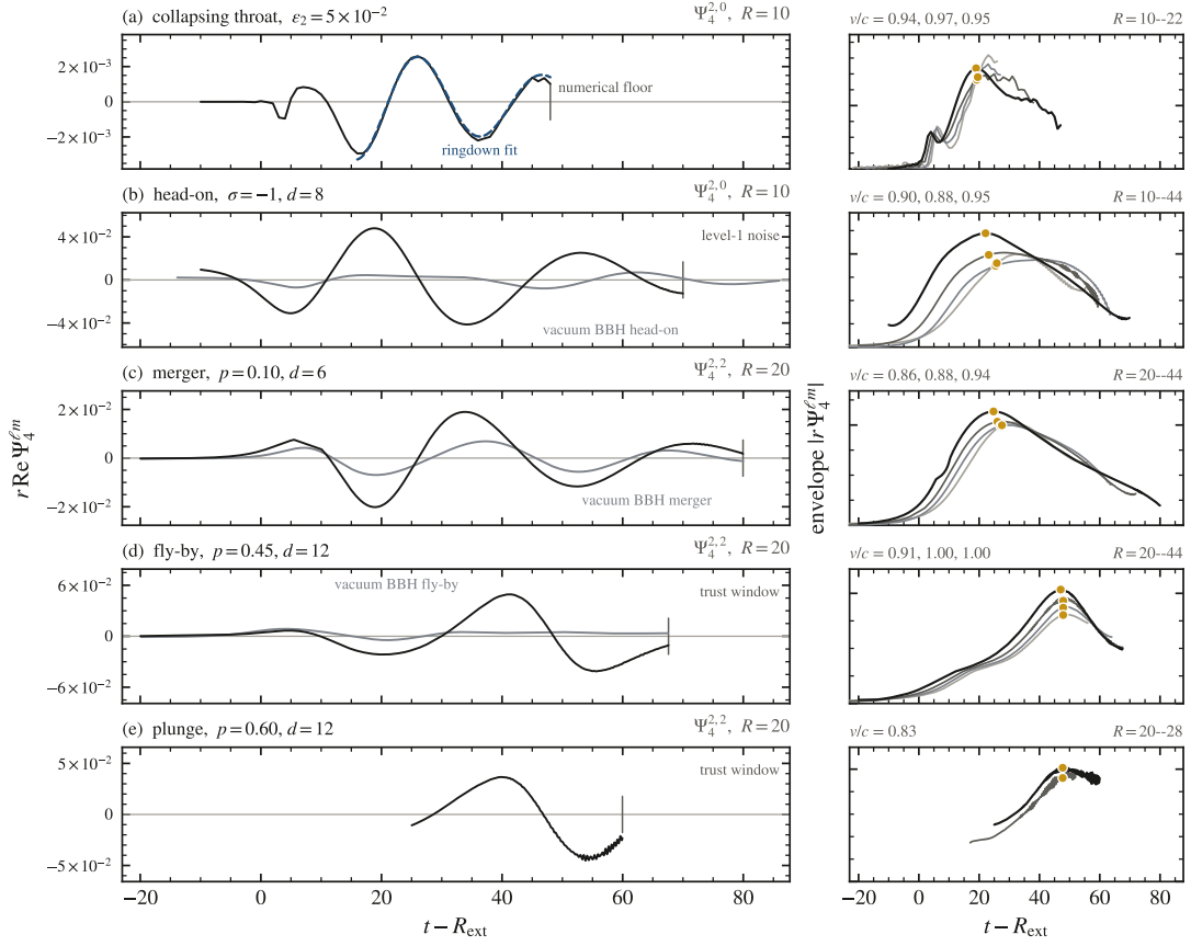
FIG. 8. The waveform gallery: one row per scenario on one retarded clock. Left: r \text{Re } \Psi_4 of the dominant mode at the innermost sphere, each row on its own scale; row (a) is the \varepsilon_2 = 0.05 arm, with the ringdown fit of Sec. VIII A dashed (period 20.6 M ). Caps mark where the drawn record ends: the collapsing throat before its numerical floor exceeds 14% of the burst peak; the head-on where the noise of its level-1 refinement cube reaches the sphere (from t = 80 at R \leq 20 ); the fly-by at its trust window ( t - R = 67.6 ), the plunge at its own. The merger runs through remnant ringdown, with one linear bridge across a leg seam. Grey under (b)–(d): the vacuum controls, black holes at the same d and p on bare punctures, on the same scale: the vacuum head-on rings 5.4\times lower and crests later (Sec. VIII B); the vacuum merger peaks at the drainhole merger’s retarded time, 3.0\times lower; the vacuum fly-by radiates one cycle as the holes swing away from periapsis, 6.7\times below the fly-by’s arch. Right: the amplitude envelope at every sphere on its own retarded time (ink to faint, inner to outer)—the upper envelope of |r\Psi_4| for the complex (2,2) modes, the analytic-signal envelope for the real (2,0) modes—which folds onto one curve for a signal moving at c and falling as 1/r . Gold dots: the correlated wavefront. The quoted v/c is the whole-waveform lag between neighbouring spheres (Sec. VIII E), the plunge’s the burst-peak lag: throat 0.94/0.97/0.95, head-on 0.90/0.88/0.95, merger 0.86/0.88/0.94, fly-by 0.91/1.00/1.00, plunge 0.83. Movies of the vacuum head-on and fly-by: Videos 8 youtu.be/aRWvD4W8OOg and 9 youtu.be/65_3kw4obvE .
