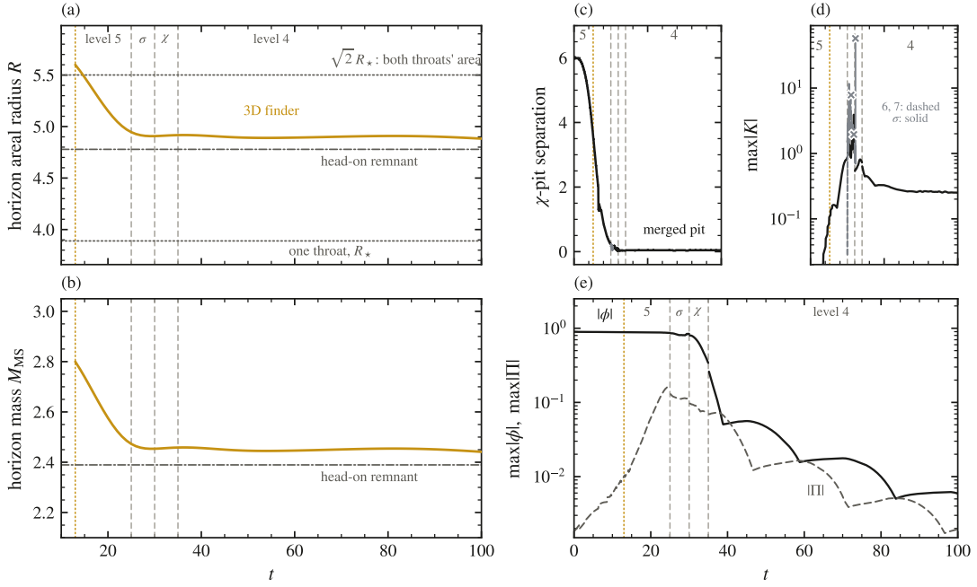
FIG. 7. The orbital merger ( d = 6 , tangential p = 0.10 , opposite signs, boosted mode-3 data) carried through its merger wall, and the black hole it settles to. One evolution composed across its legs (faint dashed rules at the restarts, t = 25, 30 and 35 ; levels named in the panels, \sigma and \chi for the two wall legs): level 5 from t = 0 , stopped at t = 26.26 as the merged core's K ran away; the \sigma_{\text{KO}} = 1.0 leg; the \chi -floor crossing leg; the level-4 settle leg to t = 100 , no NaN. (a) Areal radius and (b) Misner–Sharp mass of the common MOTs: gold, the spectral finder's history (Sec. III D), born at t = 13 and falling from above toward the head-on remnant's values (dash-dotted rules, R = 4.7787 ; M_{\text{MS}} = 2.3894 in (b)). Dotted rules in (a): one isolated throat, R_* ; \sqrt{2}R_* , both throats' area. (c) Separation of the \chi pits (grey: leg 1's overrun past its restart checkpoint). (d) The wall: \max|K| of every arm—the used legs in ink; the level-6 and level-7 diagnostic restarts (grey dashed) die at t = 29.4 and, earlier, 27.5 , each an h_{11} NaN at the core's centre with the global norms clean to the last step; the \sigma arm (grey solid) clears the K wall and dies at the same cell at t = 30.5 (death crosses); the \chi -floor and settle legs carry the history through. (e) Grid maxima of |\phi| (solid) and |\text{II}| (dashed): the field is swallowed. Gold dotted rule: horizon birth. Movie: Video 7; youtu.be/jNnMAXPjyRA .
