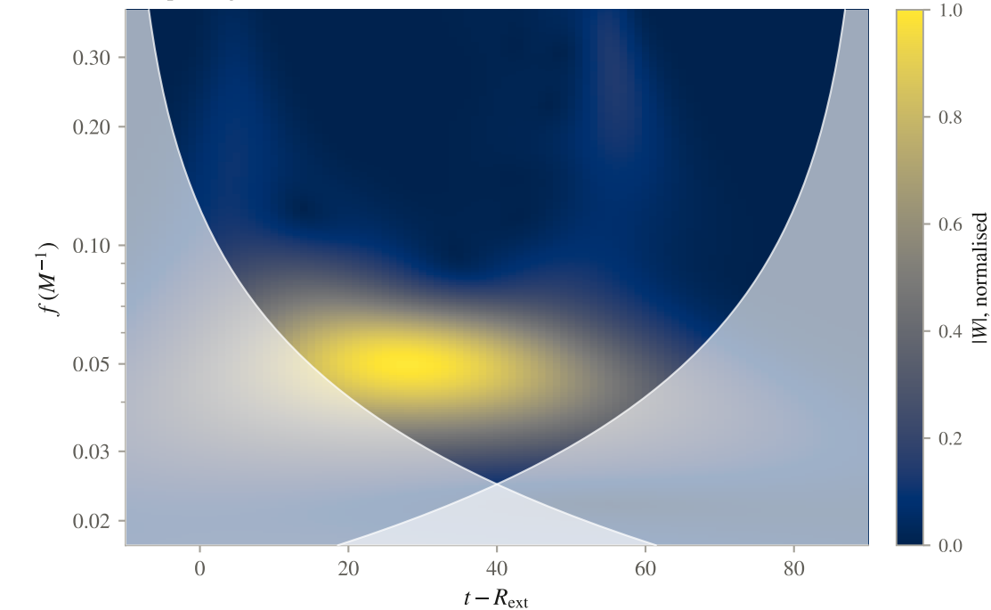
(e) spectrogram at R=10 (faded: the wavelet overruns the record)
