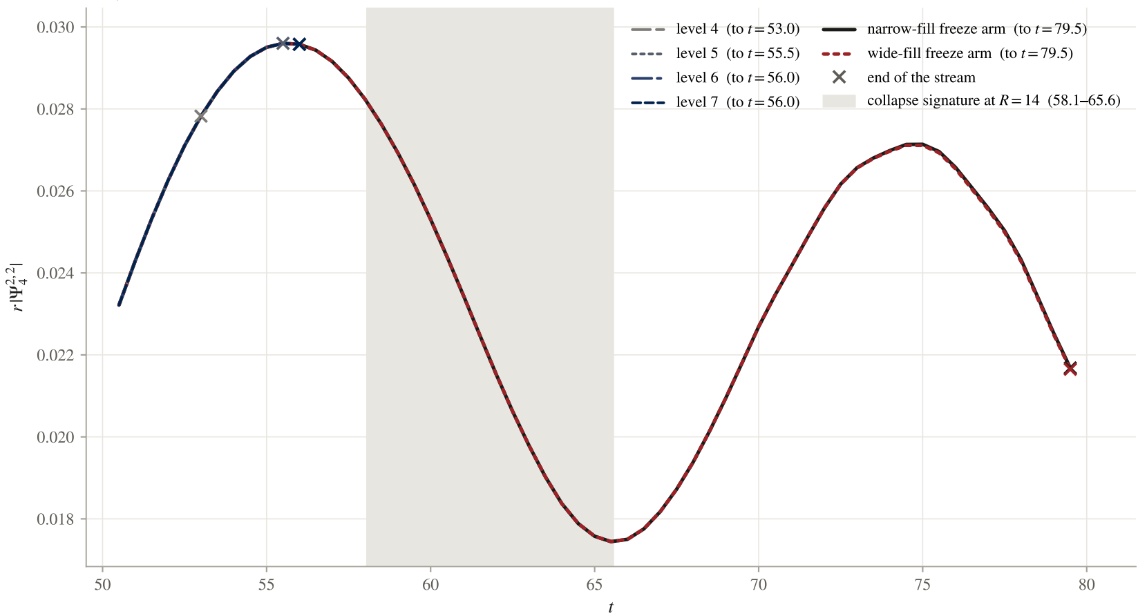
r|\Psi_4^{2,2}| at R=14 — the refinement ladder against the freeze arms
