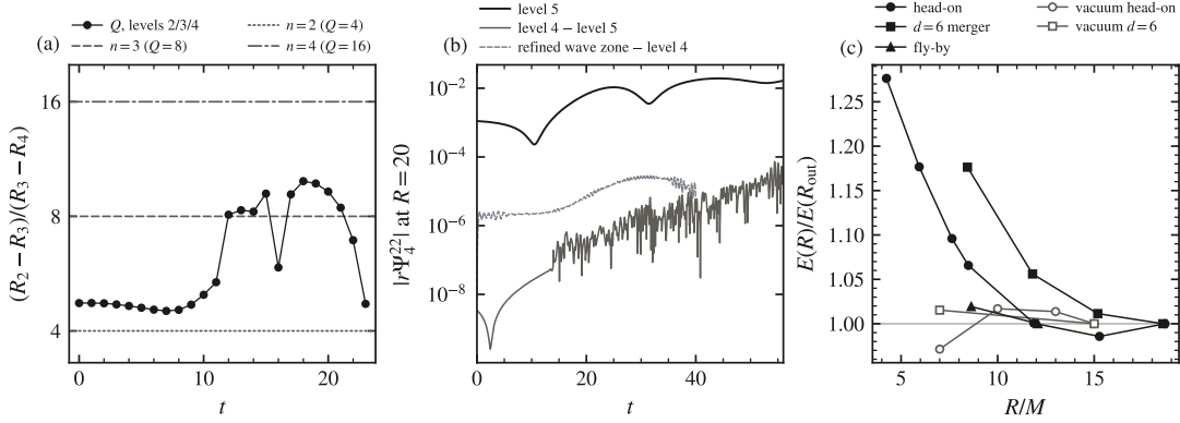
FIG. 11. Convergence. (a) The static throat from exact data at levels 2–4: the three-level factor Q = (R_2 - R_3)/(R_3 - R_4) of its minimal areal radius against the orders n = 2, 3, 4 (rules); the dip at t = 16 is one level-2 dump. (b) |r\Psi_4^{22}| at R = 20 of the d = 12, p = 0.12 pair with Bowen–York momentum (otherwise our data) at throat level 5, its difference from level 4, and the difference made by refining the wave zone to half the base cell. (c) Radiated energy on each sphere over the outermost sphere’s, against R/M : the head-on, the d = 6 merger and the fly-by (ink) and two vacuum controls (grey). The outcome: the scheme converges at order 3.0–3.3, a binary’s waveform is resolved to 0.4% of its peak, and the energy converges in extraction radius.
