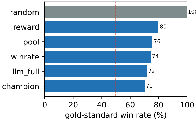
Gold beats every learned agent
