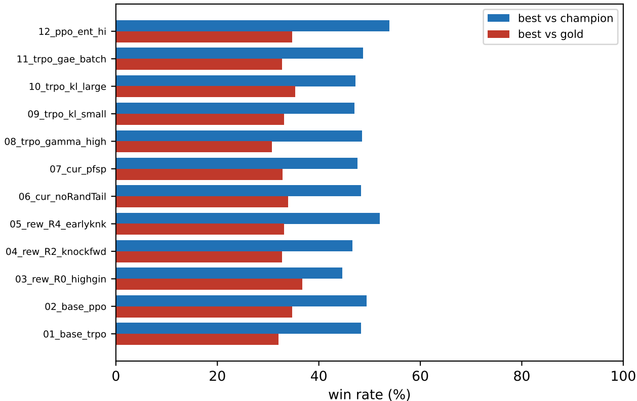
Phase-6: best win-rate per sweep cell (mean over seeds)
