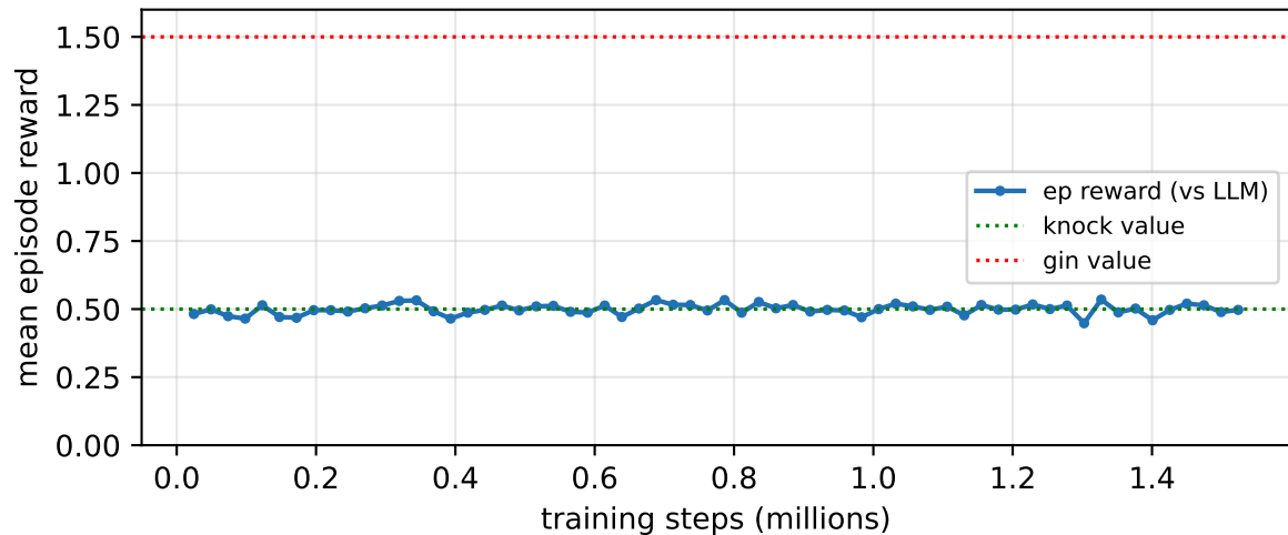
RL-vs-LLM: episode reward stays at the knock value
