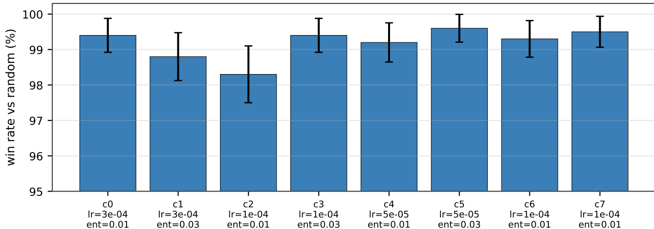
Phase-1 sweep: win rate per HP config (1000 eval episodes, 95\% CI)
