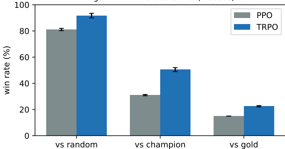
Algorithm: TRPO beats PPO (2 seeds)
