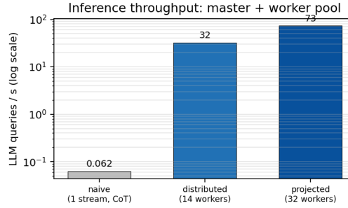
Figure 4: Aggregate LLM-query throughput. The master + worker pool with the terse prompt reaches \sim 32 queries/s on 14 workers (measured) and scales to the 32-worker target, versus \sim 0.06 q/s for a single-stream chain-of-thought loop.
