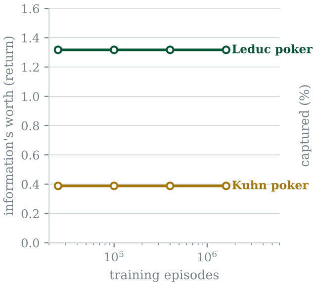
(a) Worth is fixed by the game
