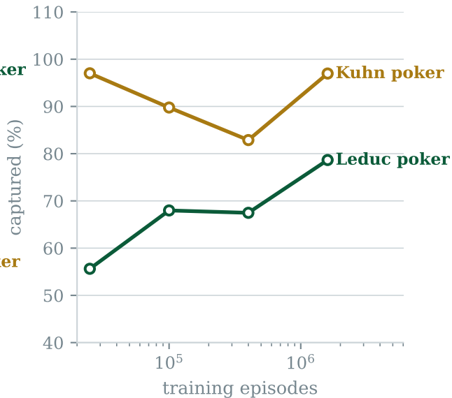
(b) The share banked grows with budget
