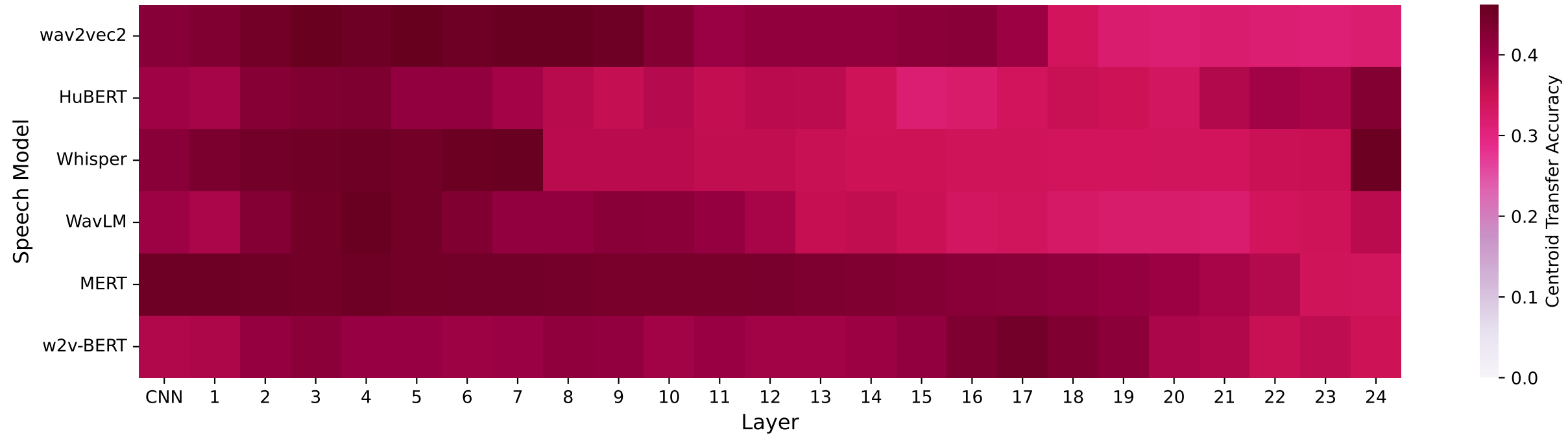
Centroid Transfer Accuracy per speech layer (IEMOCAP transcripts, BERT base)
