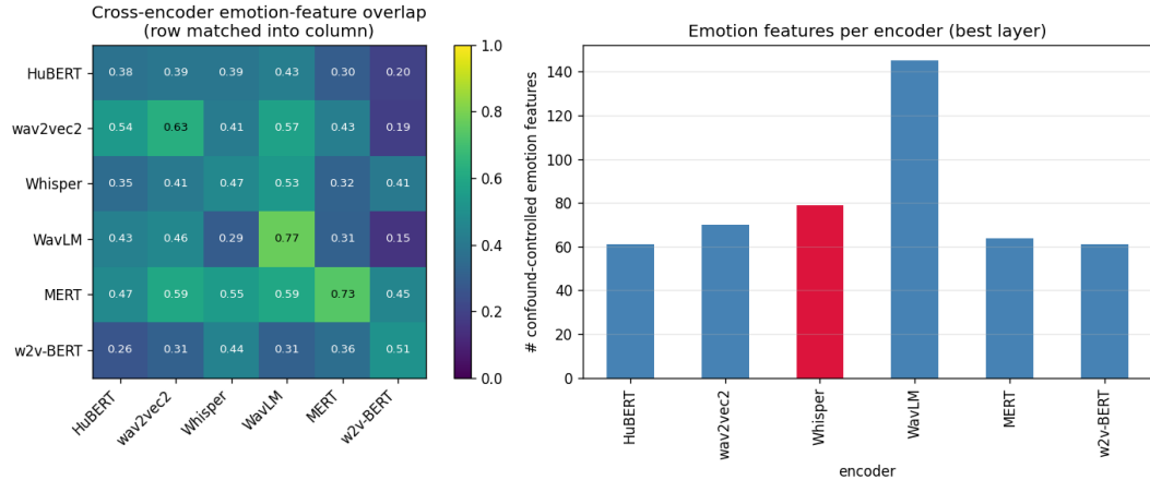
Figure 4: Cross-encoder picture. Left: how much each encoder’s emotion features overlap with every other’s — Whisper is not an outlier. Right: number of clean emotion features per encoder at its best layer.
