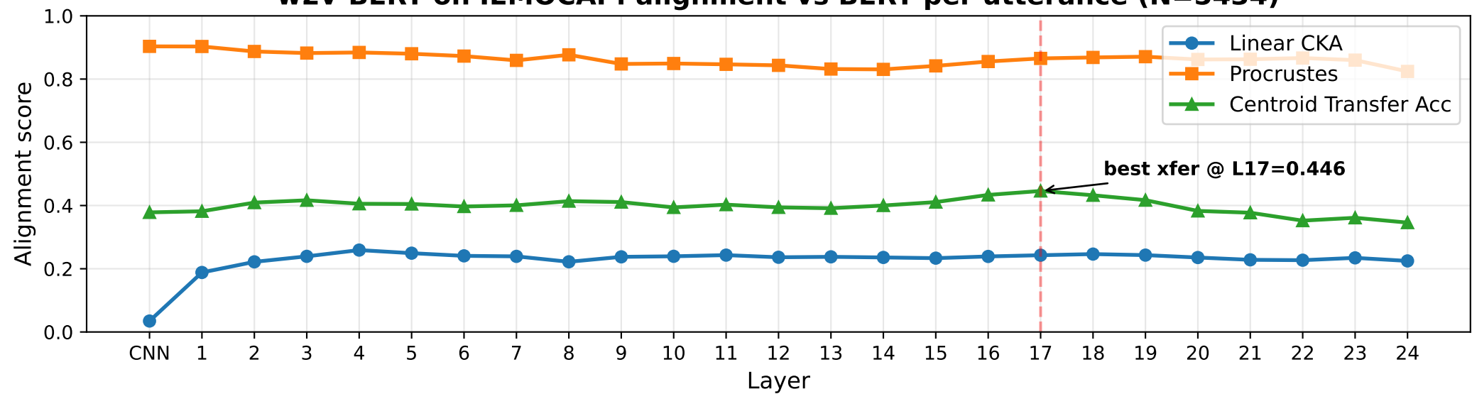
w2v-BERT on IEMOCAP: alignment vs BERT per utterance (N=5434)
