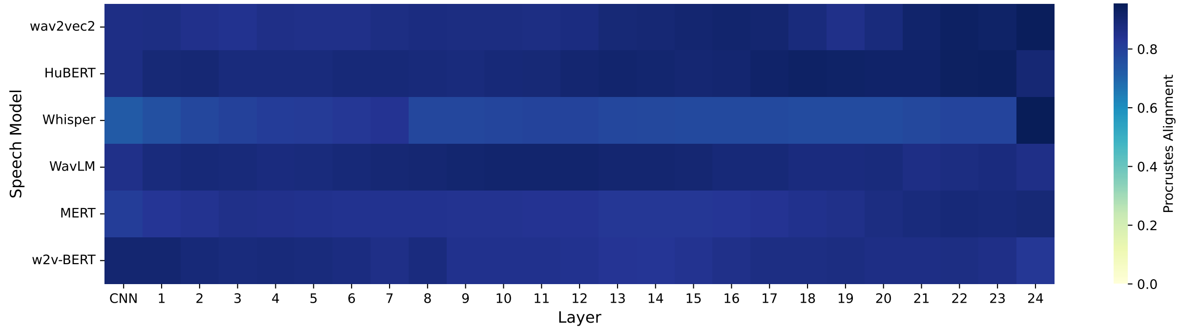
Procrustes Alignment per speech layer (IEMOCAP transcripts, BERT base)
