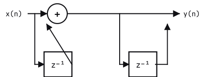
DIRECT FORM I - TWO DELAY CHAINS
