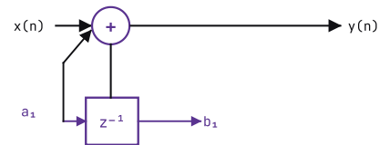
DIRECT FORM II - ONE
