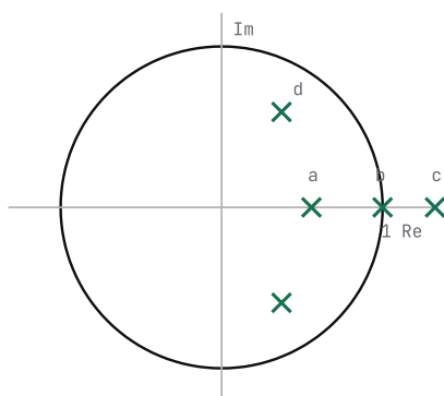
the z -plane — poles marked ×
