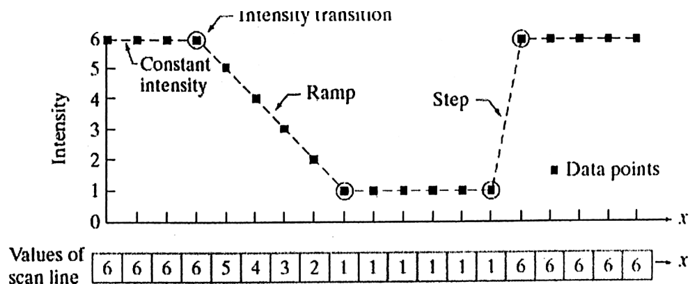
Fig.6 — the gray-level profile, with the constant region, the ramp and the step labelled, and the values of the scan line written underneath.
