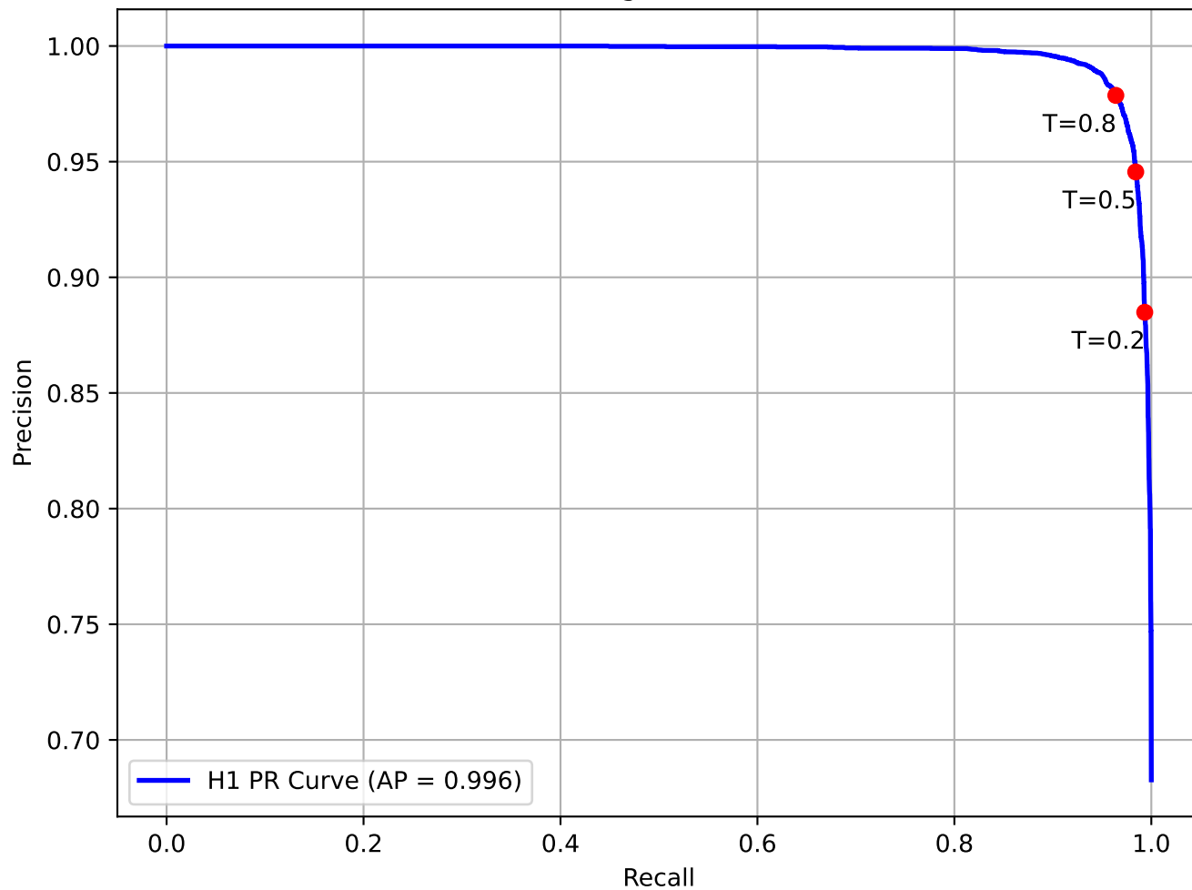
H1 Triage PR Curve
