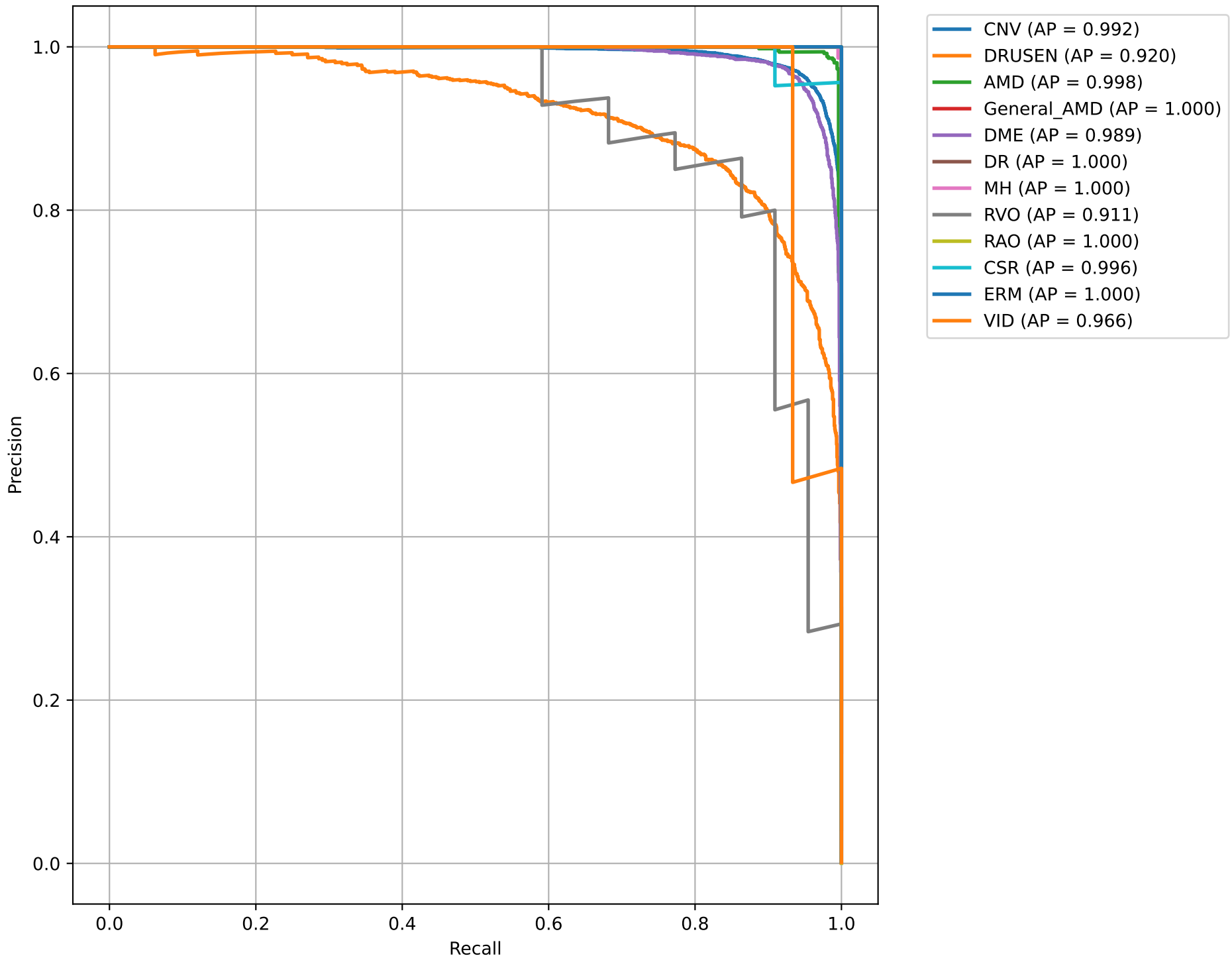
H2 Granular Pathology PR Curves
