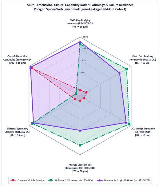
Figure 2: Multi-Dimensional Clinical Capability Radar Benchmark (Polygon Spider-Web). Clinical boundary accuracy and failure resilience across the 6 primary anatomical challenges. (Red Dashed) Commercial Solix heuristic collapses on cup bridging, wedge penetration, and tilt. (Green Dash-Dot) Bi-Planar achieves high accuracy across challenges 1–5, but collapses on Axis 6 (slice continuity). (Purple Solid) Dense 3D U-Net forms a complete, well-rounded envelope encompassing all 6 clinical challenges.
