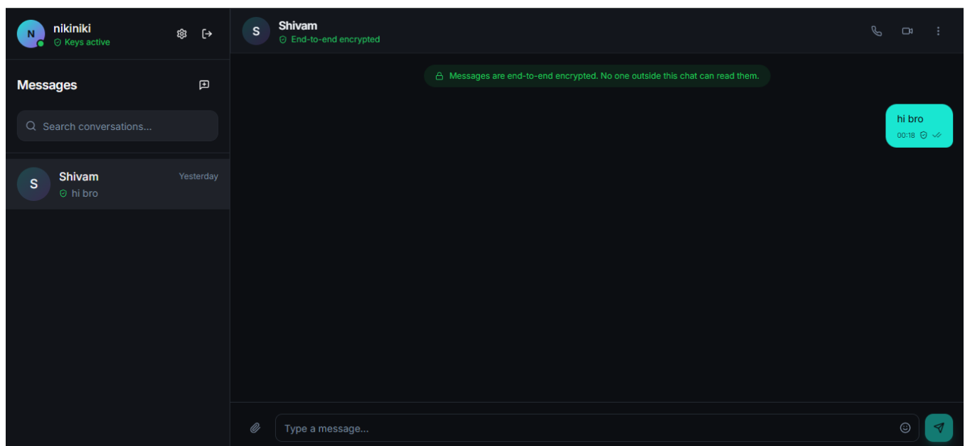
Fig 6.9.1 Chat Application
