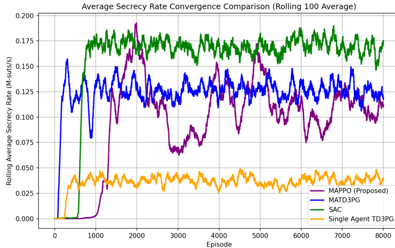
Fig. 2. Convergence comparison showing the rolling 100-episode average secrecy rate (M-suts/s) for all four RL algorithms (MAPPO, MATD3PG, SAC, and Single Agent TD3PG) on the Week 9 system model.
