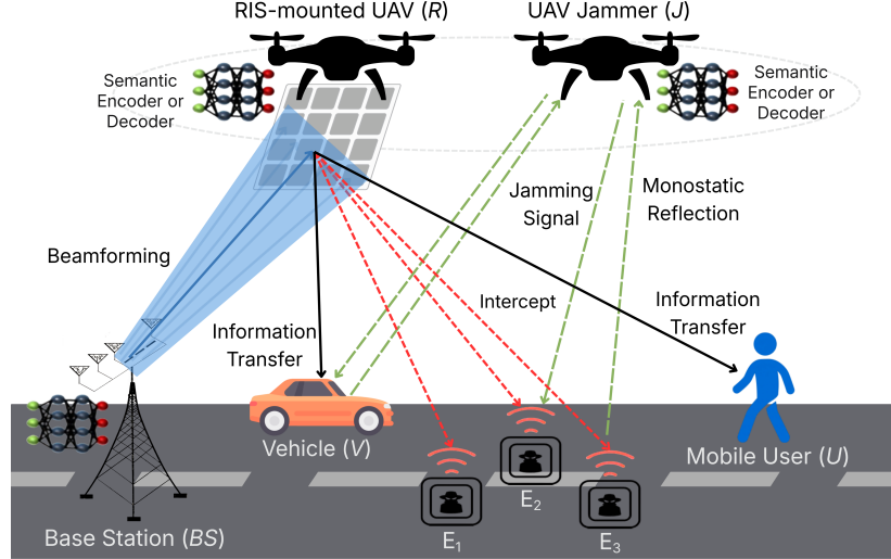
Fig. 1. System model of the secure semantic-aware ISAC dual-UAV network featuring RIS reflection, full-duplex jamming, PD-NOMA, and monostatic radar sensing.
