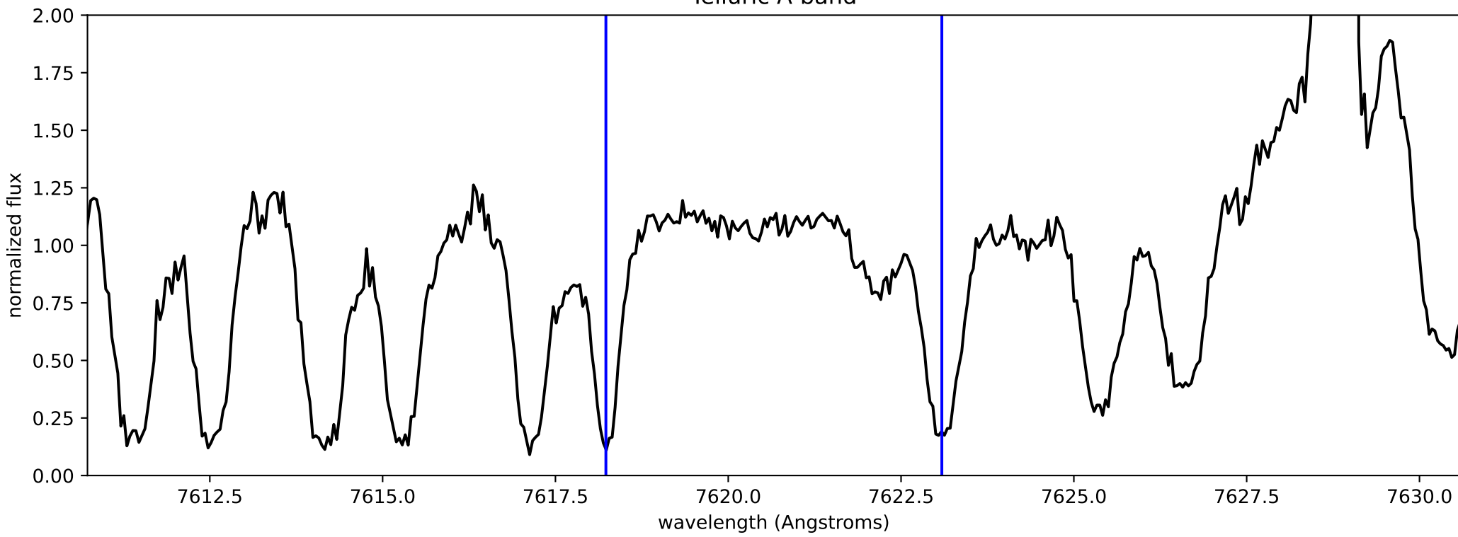
Telluric A-band
