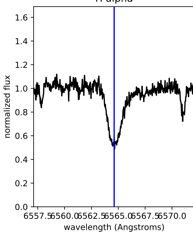
H alpha
