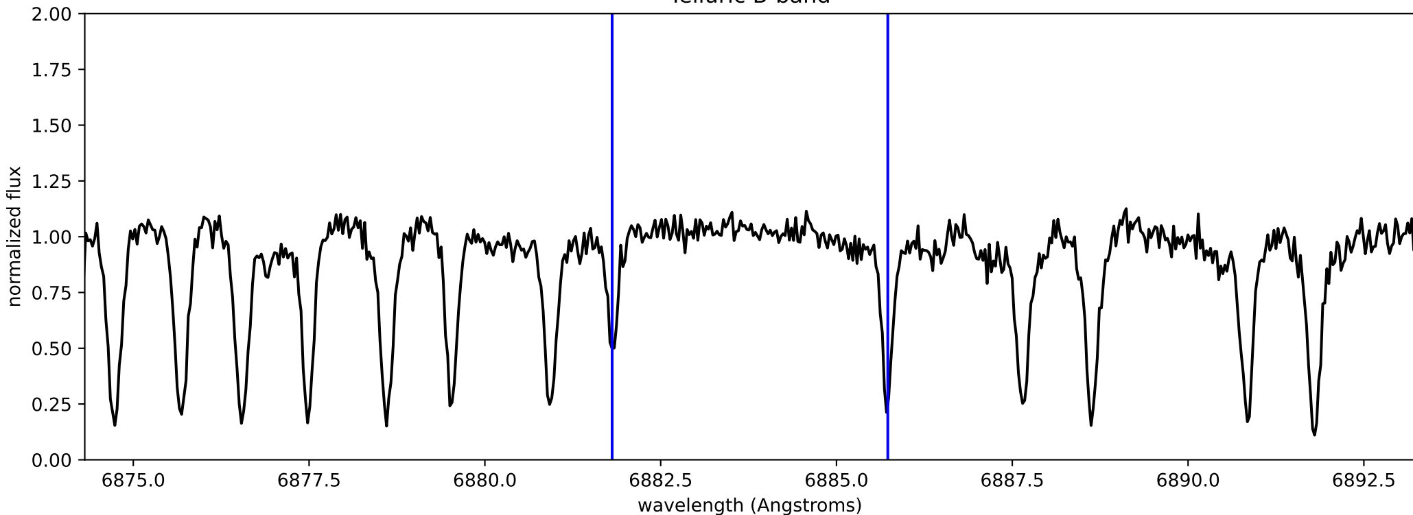
Telluric A-band
