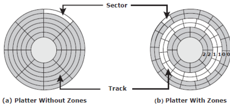
Figure 2-9: Zoned bit recording
