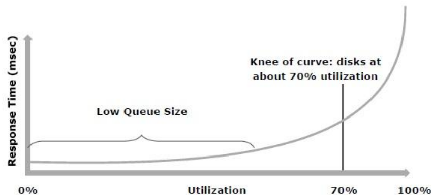
Figure 2-10: Utilization vs. Response time
