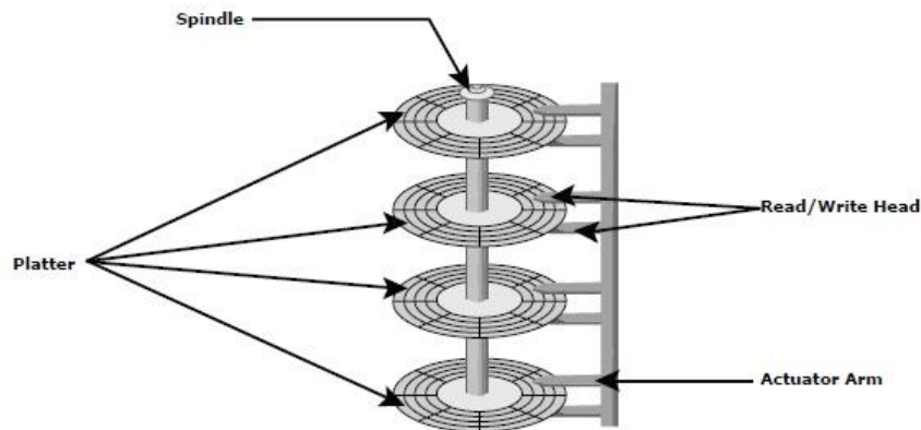
Figure 2-4: Actuator arm assembly
