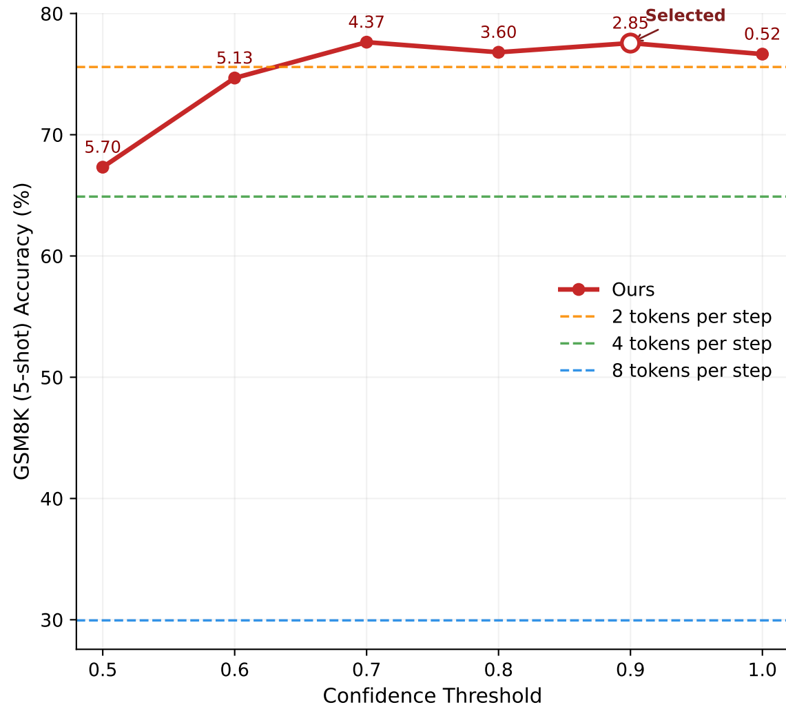
(a) Accuracy vs Threshold
