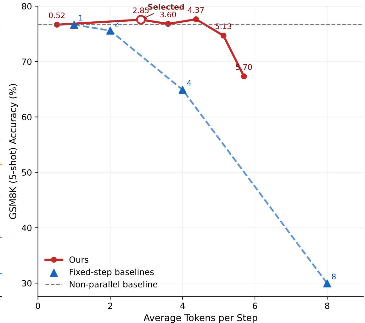
(c) Accuracy vs Average Tokens/Step
