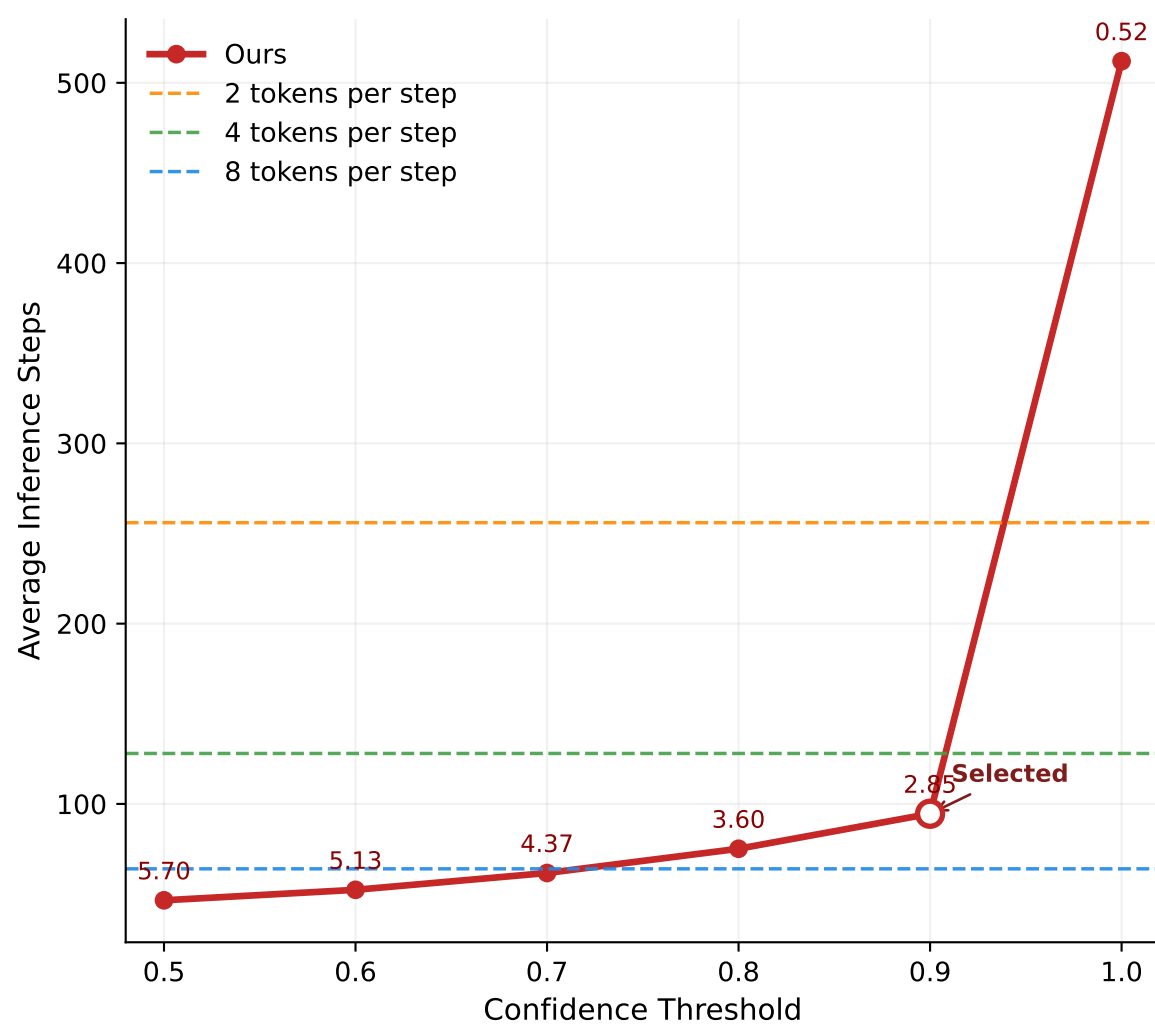
(b) Inference Steps vs Threshold
