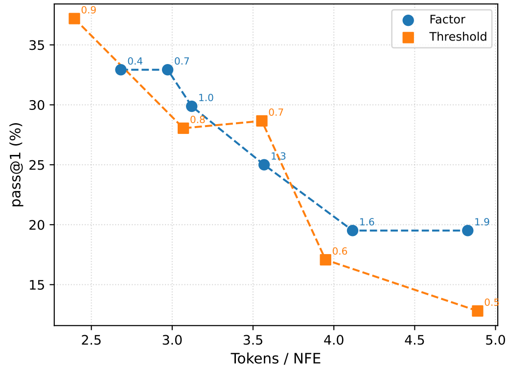
HumanEval — Factor vs Threshold (batch size 1)
