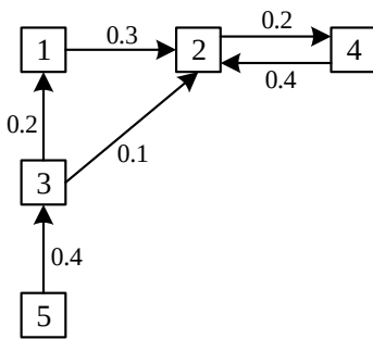
FIGURE 2. An Independent Cascade model with 5 nodes.
