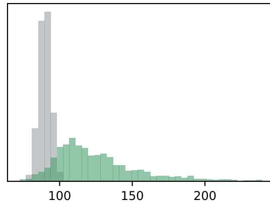
baseline 91% real OOD (shift +7.1z)
