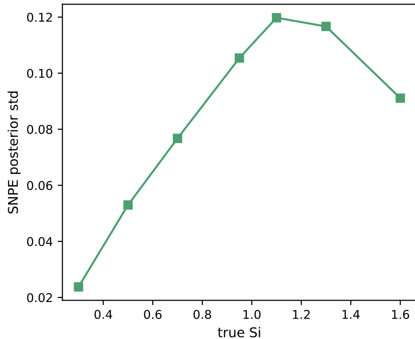
posterior width grows where S_i is unresolved
