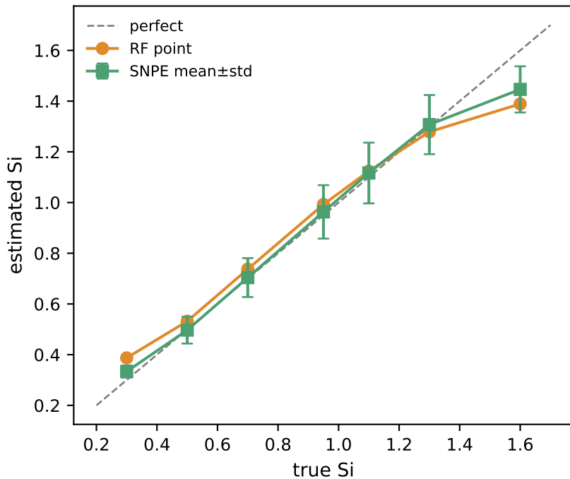
RF shrinks at extremes; SNPE stays honest
