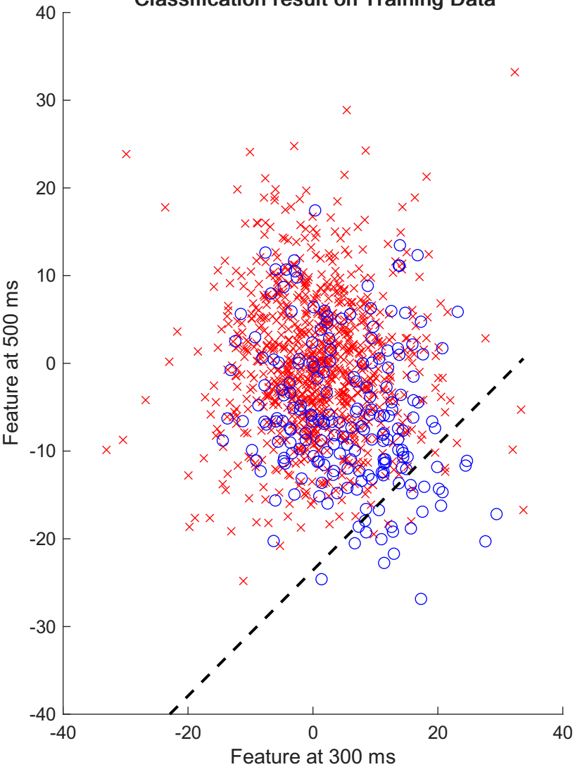
Classification result on Training Data
