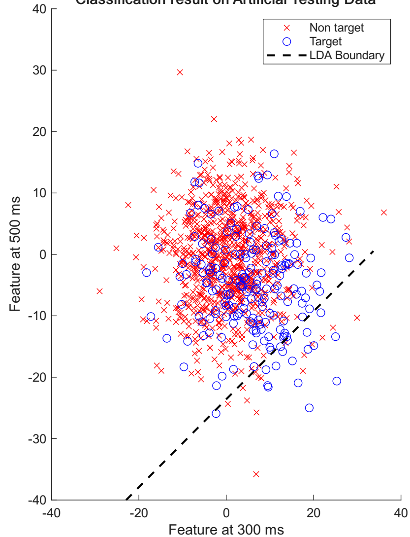
Classification result on Artificial Testing Data
