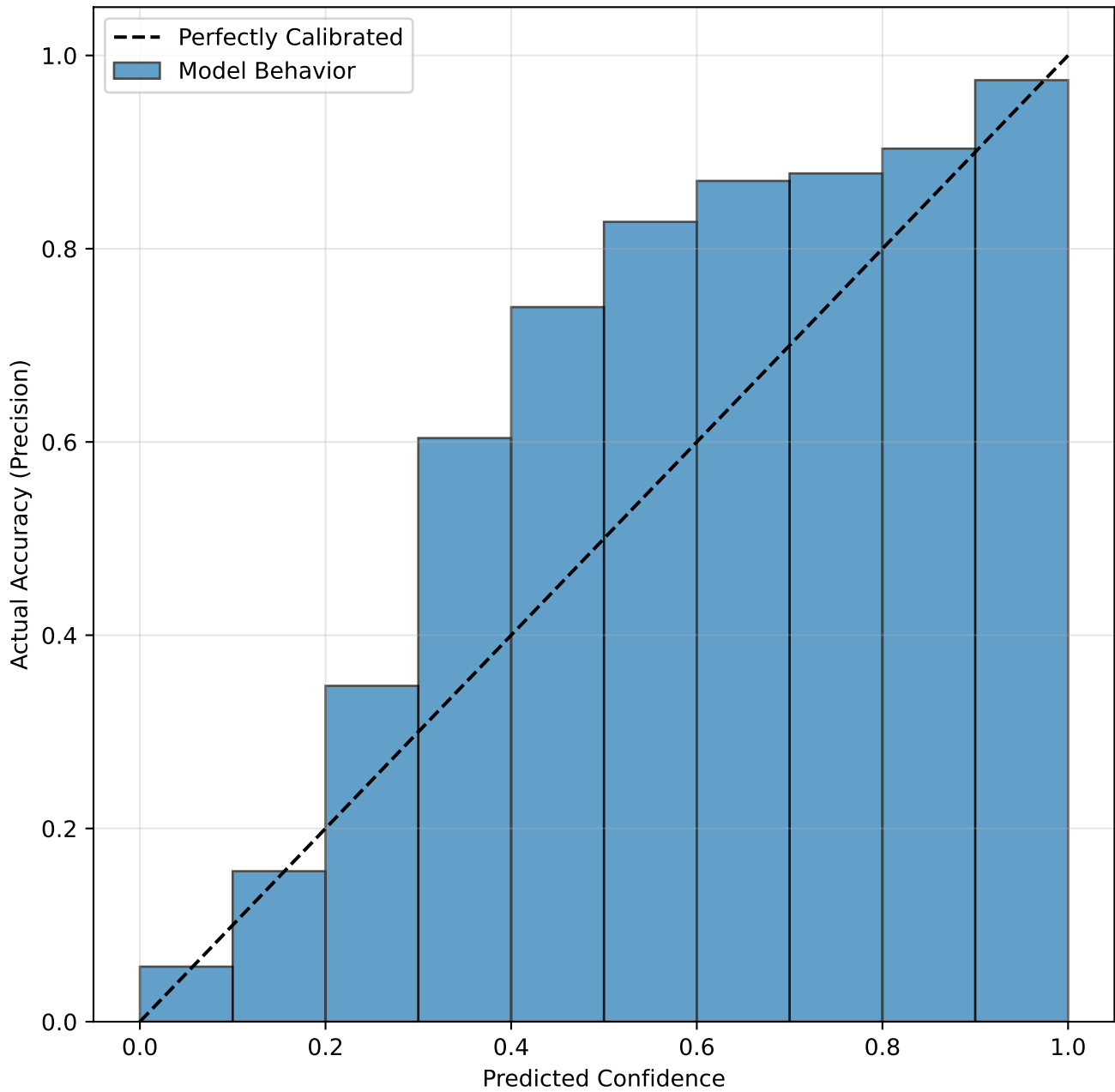
YOLOv1 Confidence Calibration Plot
