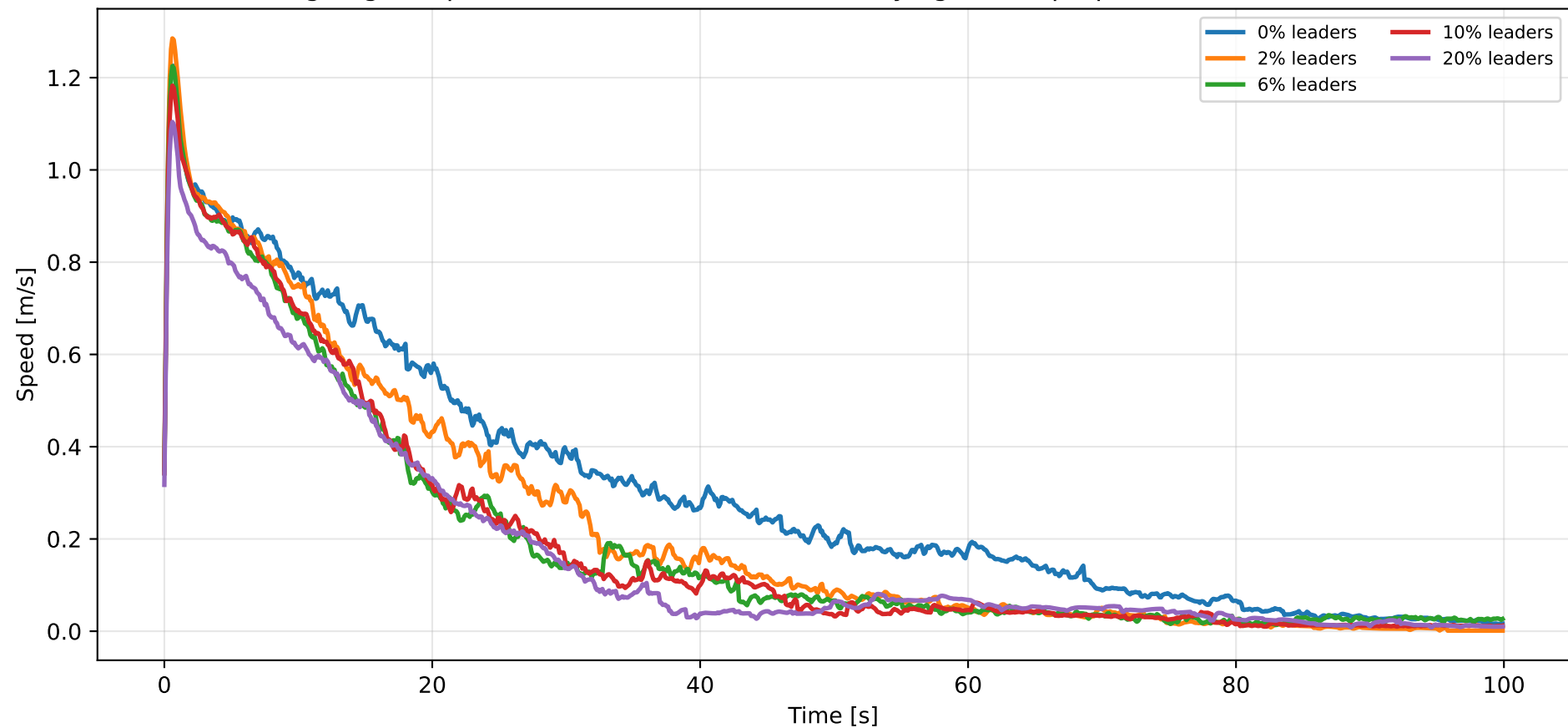
Average agent speed over time (Fire enabled, varying leader proportion; mean of 30 runs)
