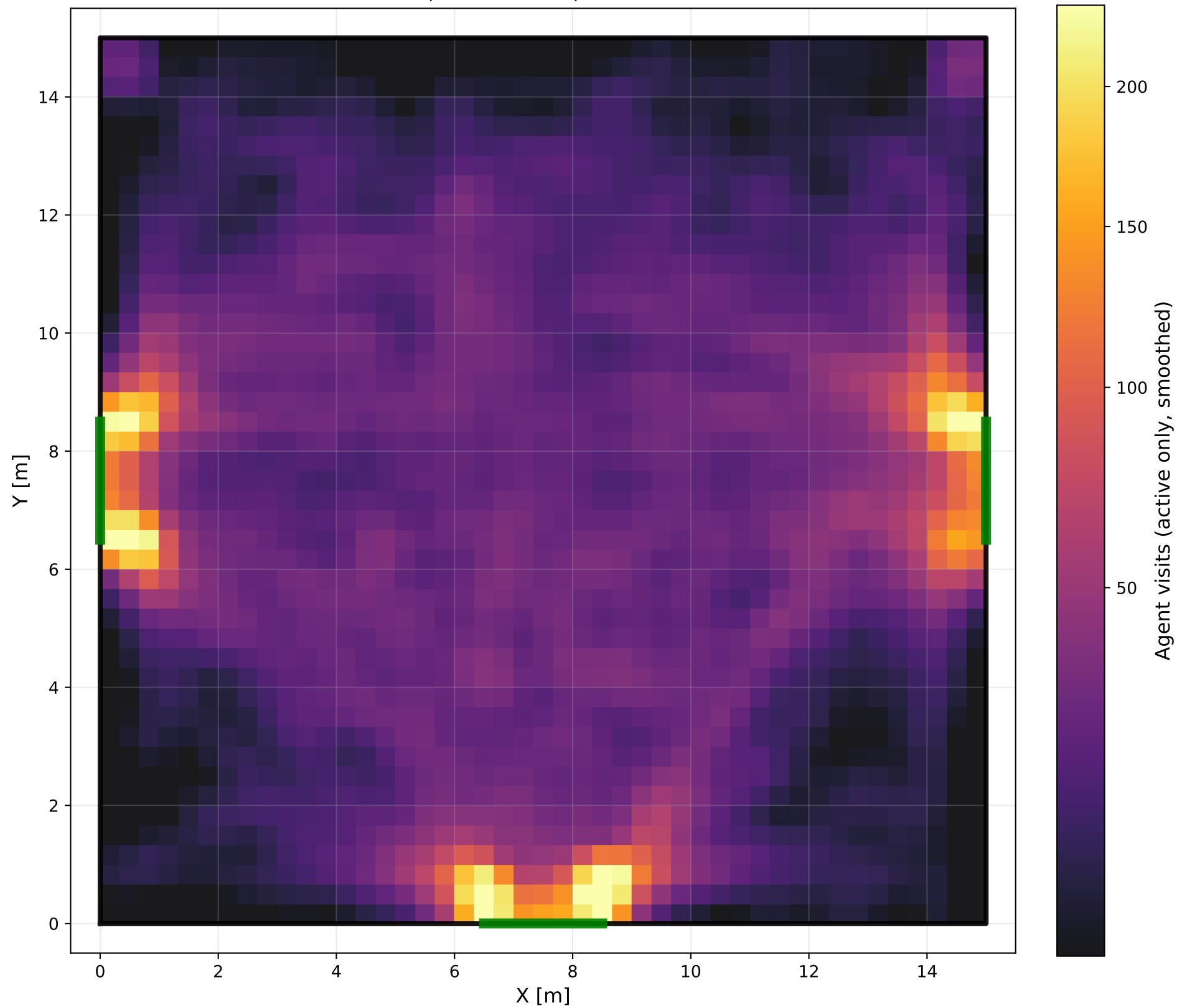
Agent Position Heatmap No Fire, Three Exits, 20% Leaders
