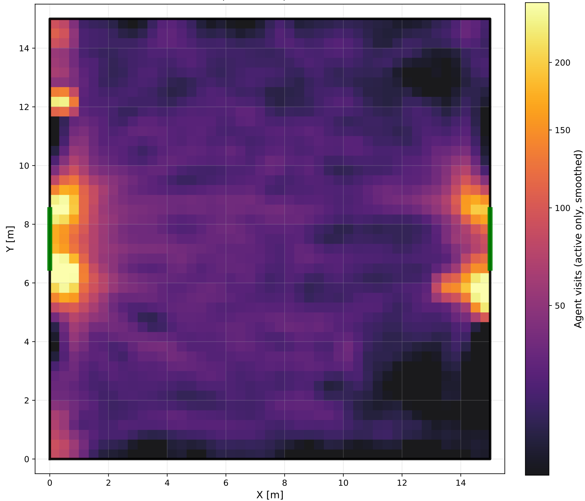
Agent Position Heatmap No Fire, Two Exits, 6% Leaders
