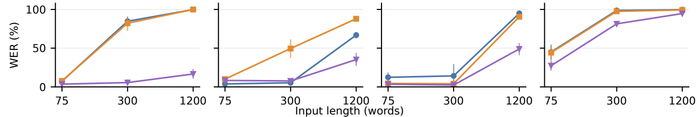
CosyVoice3
