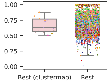
Group N LOBO macro-F1 (3-class) p = 0.82 , \text{rbc} = -0.03
