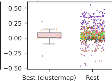
Group N LOBO macro-F1 (3-class) p = 0.82 , \text{rbc} = -0.03
