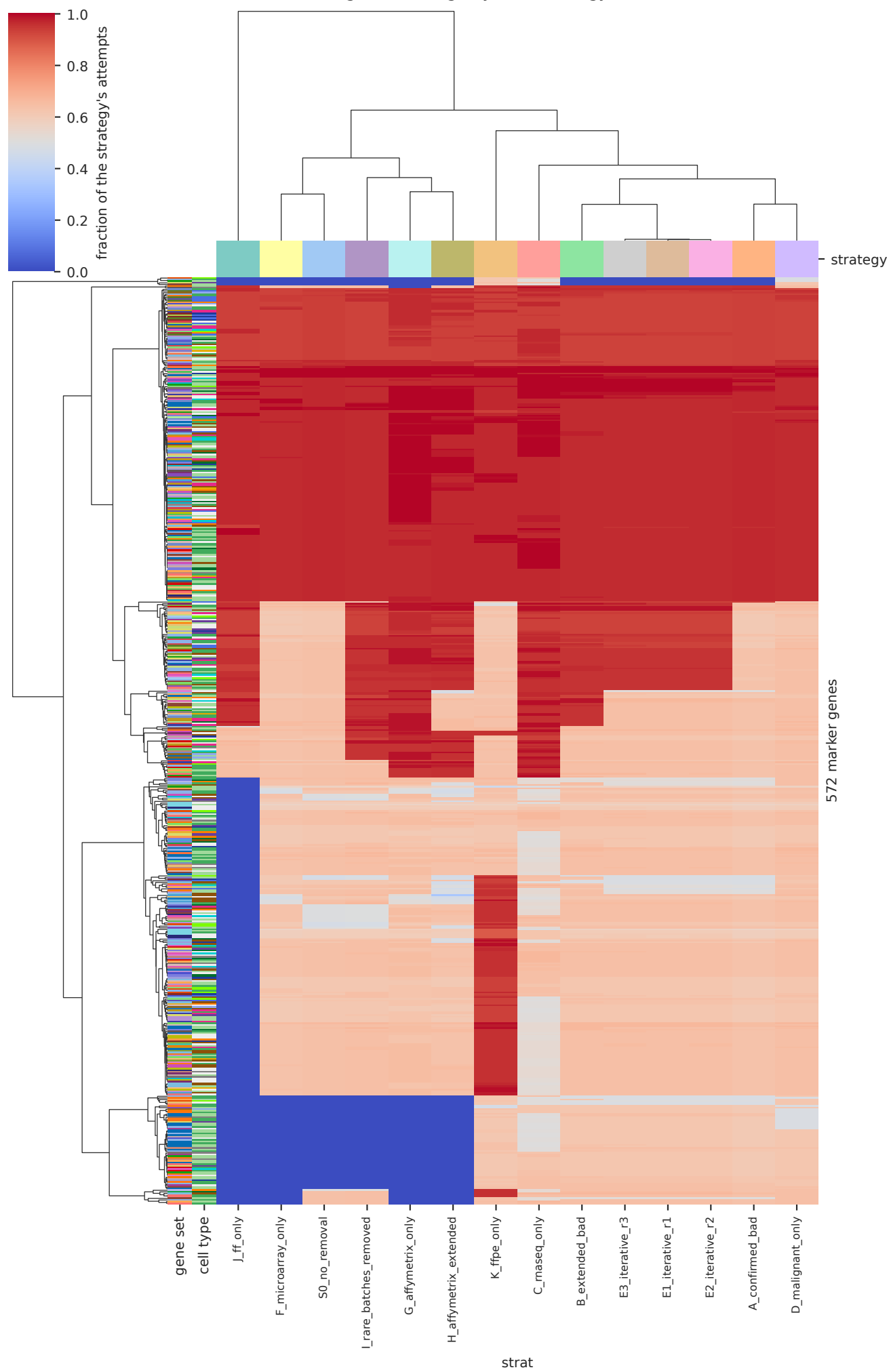
Marker gene coverage by filter strategy
